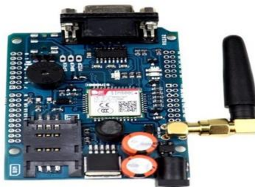
Figure13: GSM SIM800C
