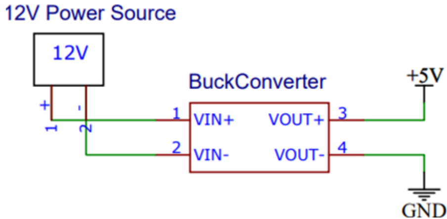
Figure 4: Power supply
