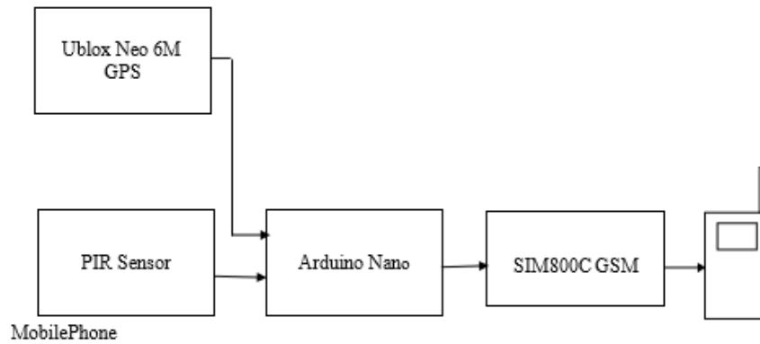
Figure 2: Block diagram of Intruder Monitoring
