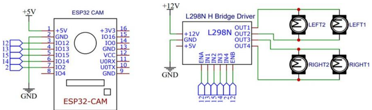
Figure 5: ESP32 CAM and L298N Pin descriptions
