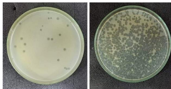
Figure 4: Double Layer Agar Method Showing Plaques of Different Size of Bacteriophages.
