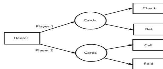
Figure 32: AKQ Game
