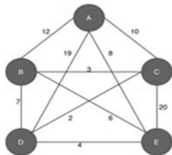
Figure 1: Travelling Salesman Problem
