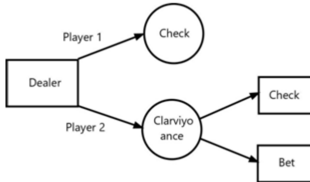
Figure 29: Clairvoyance Game
