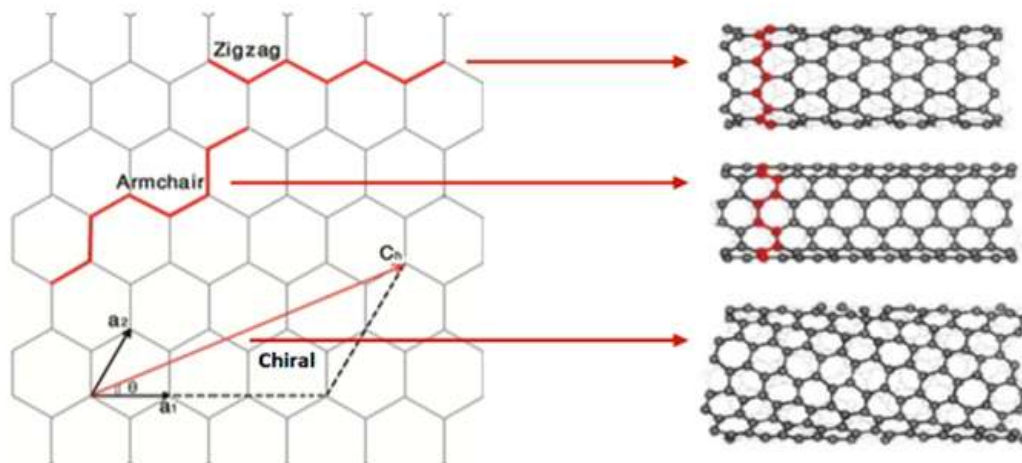
Figure 3: Schematic Diagram Showing Zigzag, Armchair and Chiral Carbon Nanotubes
