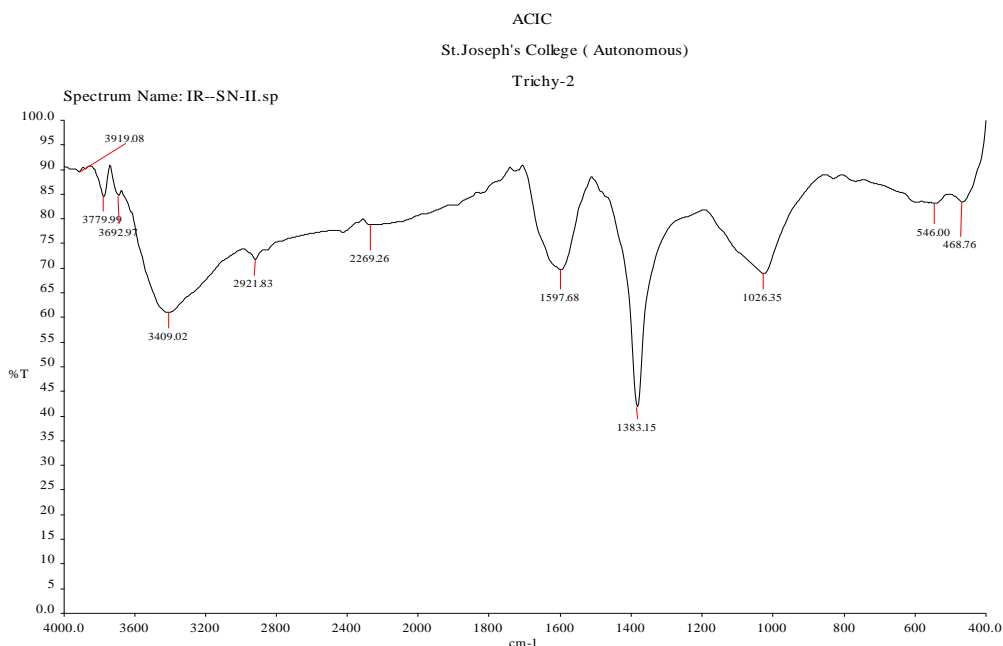
Figure 5: FTIR of the Band Representing Various Functional Groups.
