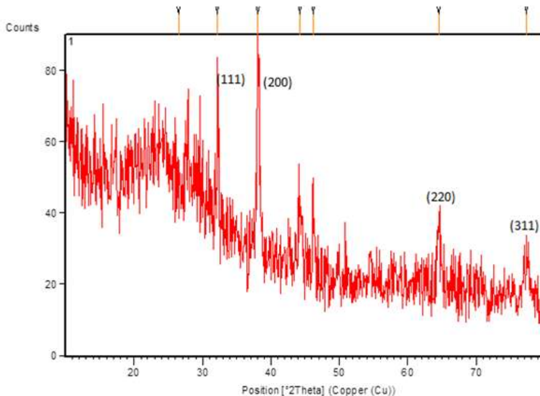
Figure 3: XRD Pattern of Synthesized Silver Nanoparticles (Peaks Corresponding To Silver).
