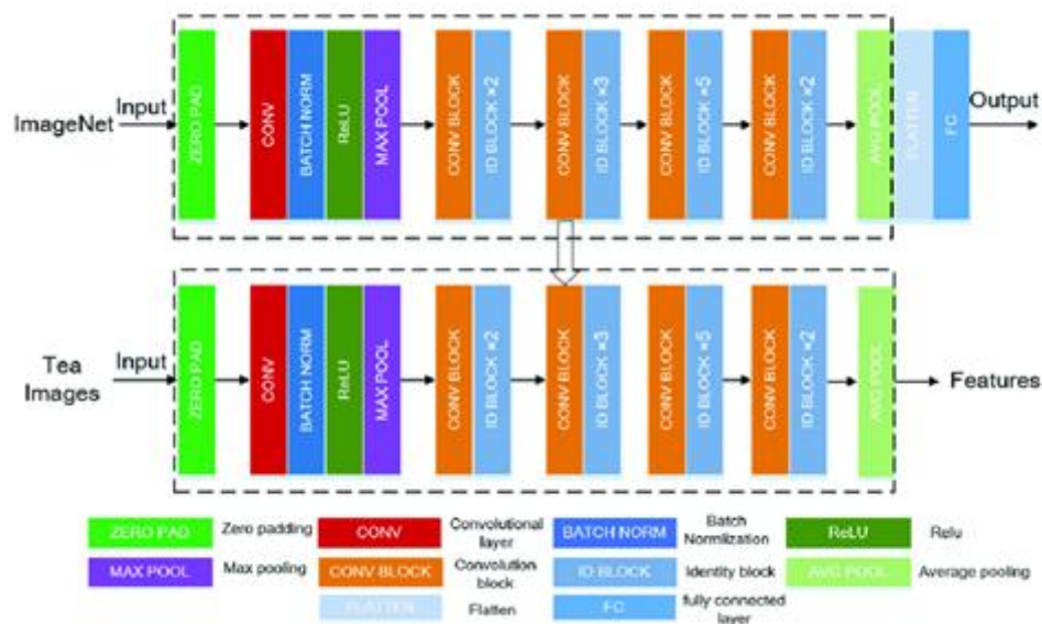
Figure 14: The Framework of ResNet50
