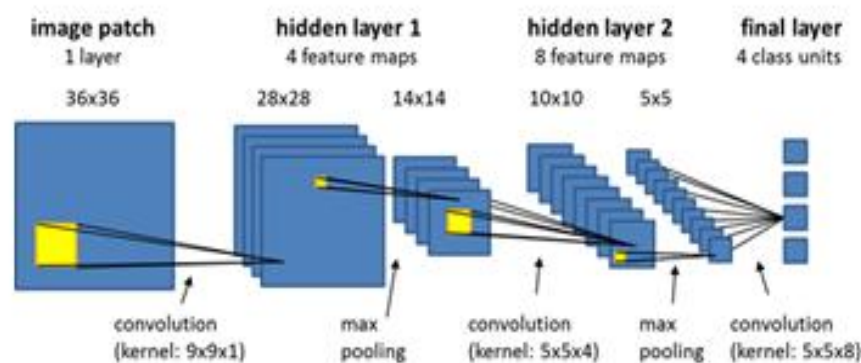
Figure 11: Convolutional Neural Network Layers
