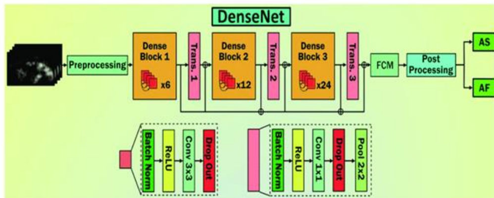
Figure 15: The Architecture of Dense Net
