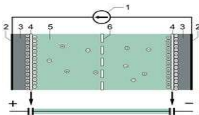
Figure 5: Typical construction of a supercapacitor: (1) power source, (2) collector, (3) polarized electrode, (4) Helmholtz double layer, (5) electrolyte having positive and negative ions, (6) separator.
