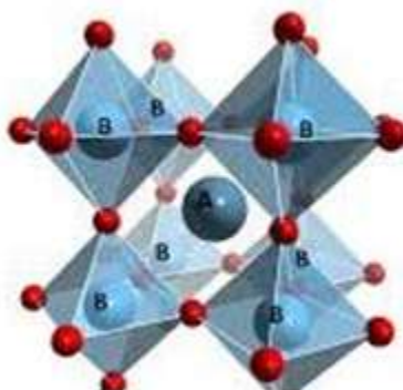
Figure 1: Perovskite Structure
