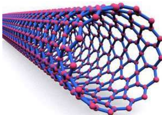
Figure 3: Carbon Nanotube
