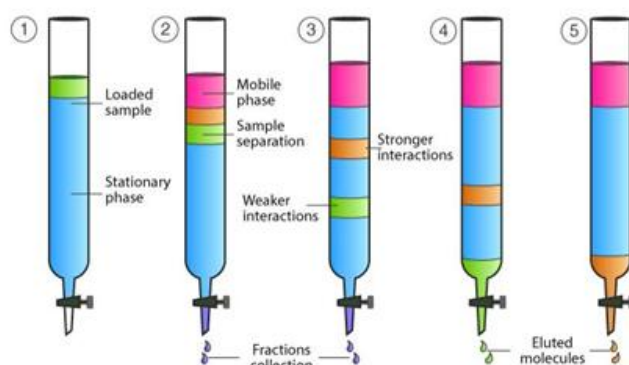
Figure 3: Column Chromatography
