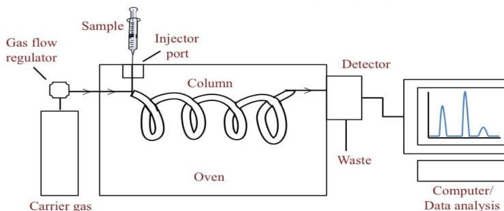
Figure 8: Gas Chromatography
