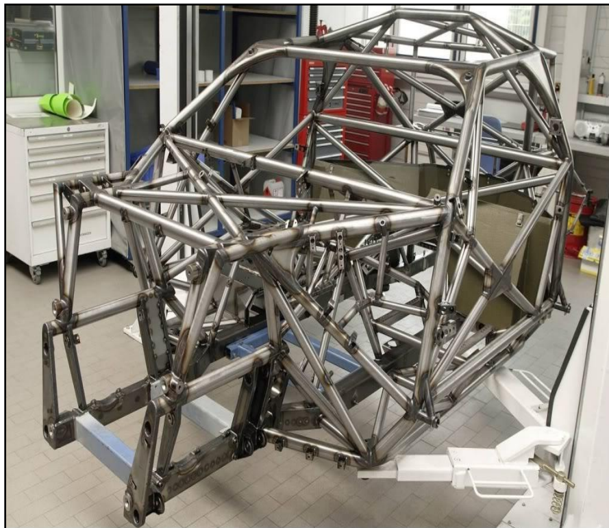
Figure 2: Tubular Chassisframe
