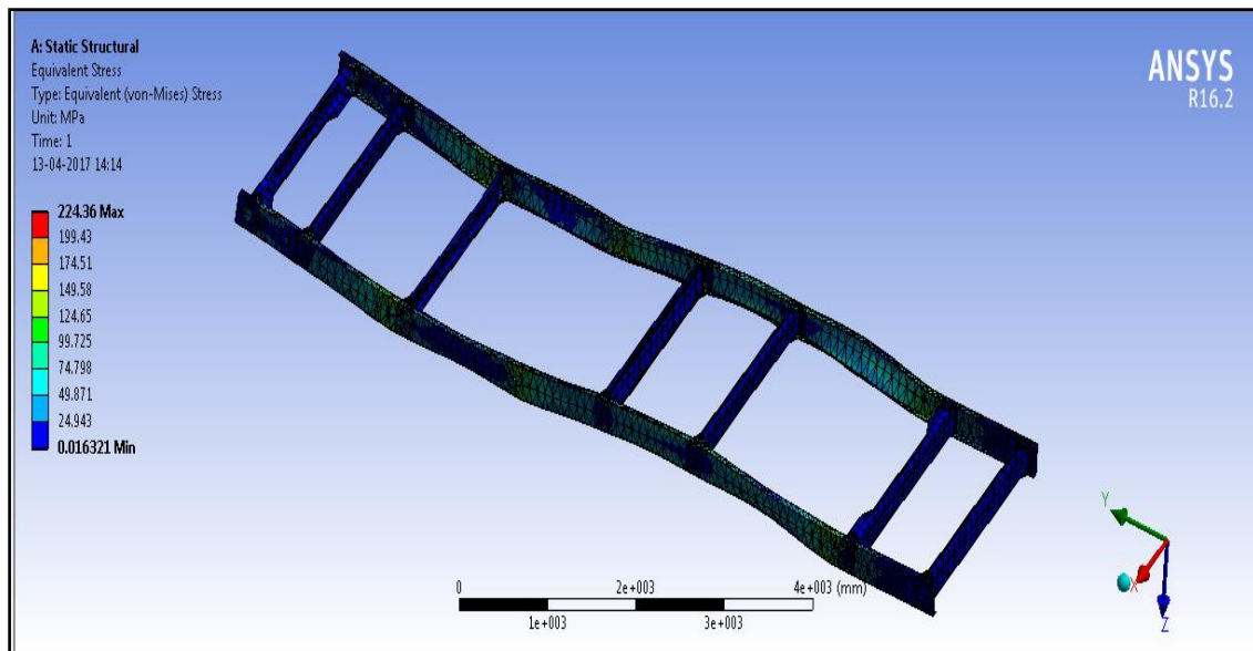
Figure 15: Stress variations in Optimized Chassis Frame with Channel Cross Section
