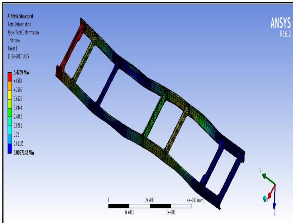
Figure 15: Deformation in Optimized Chassis Frame
