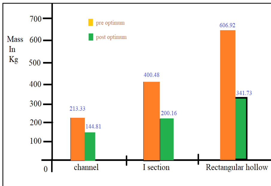
Figure 12: Reduction in Mass after Optimization
