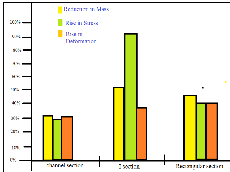
Figure 13: Reduction in Mass, Rise in Stress and Rise in Deformation for Different Cross-Sections.
