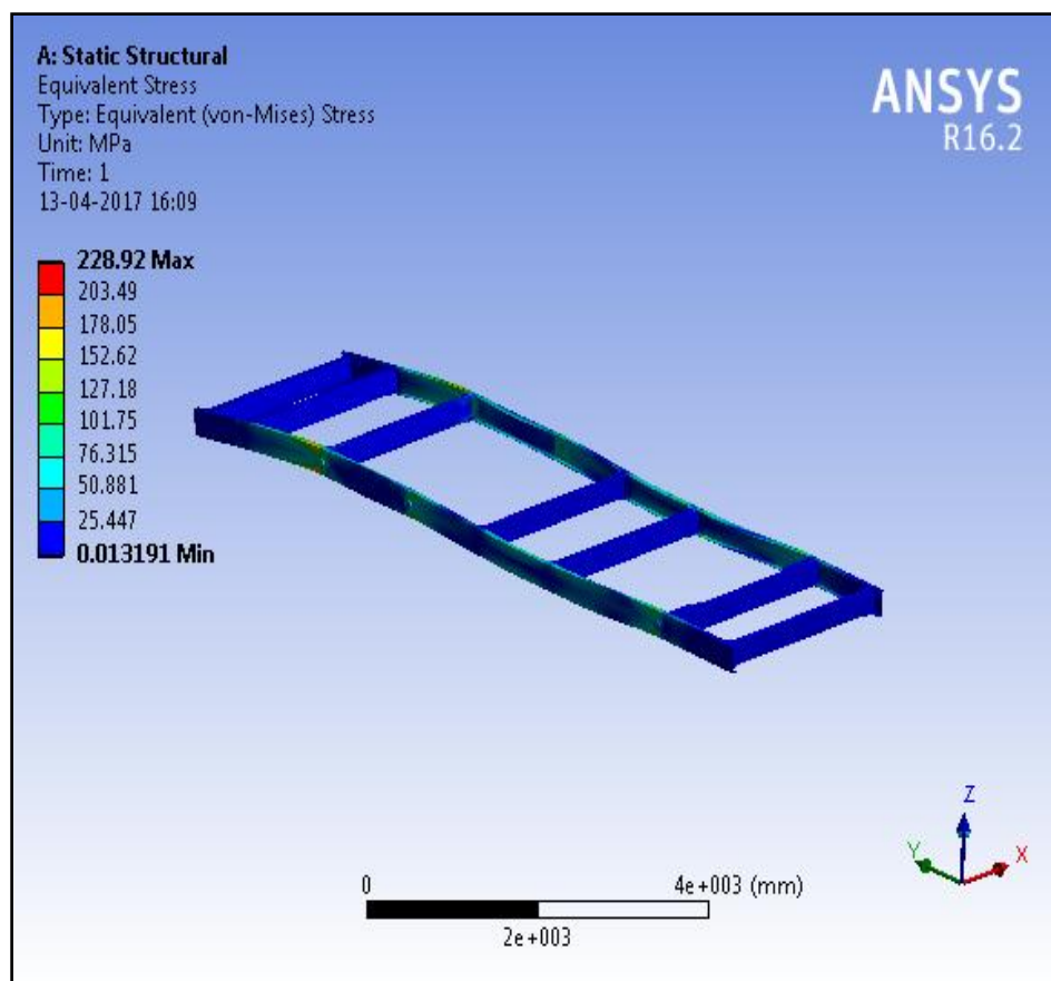
Figure 6: Stress Distributions of C-section
