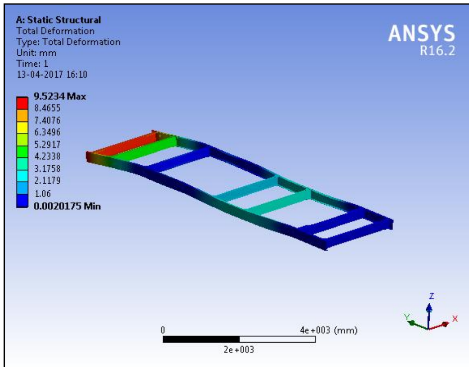
Figure 7: Displacement Pattern of C-section
