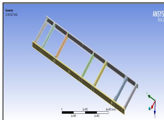
Figure 14: Optimized C-Section chassis frame
