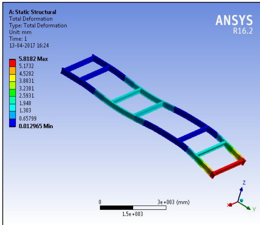
Figure 9: Displacement Pattern of I-Section
