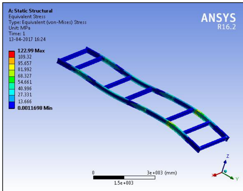
Figure 8: Stress Distributions of I-Section
