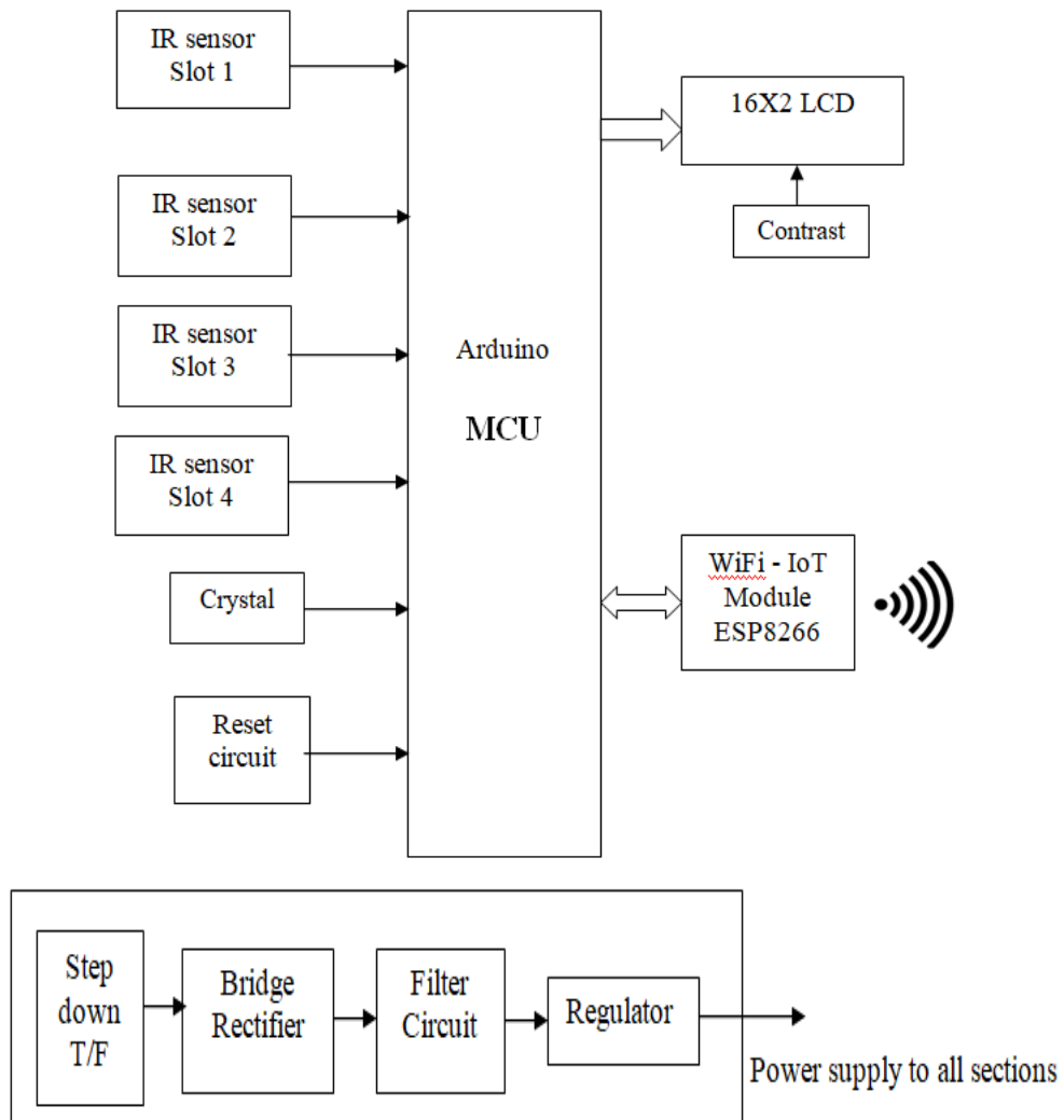
Figure 3: Block Diagram
