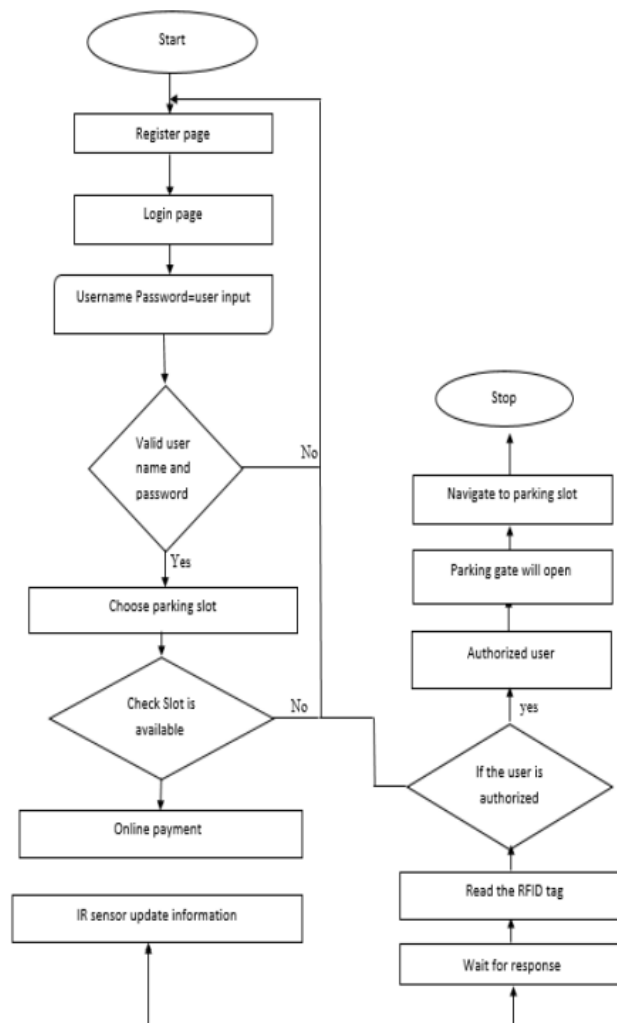
Figure 4: Algorithm
