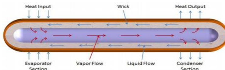
Figure 2: Heat Pipe [2]
