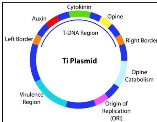
Figure 1: Schematic representation of Ti plasmid
