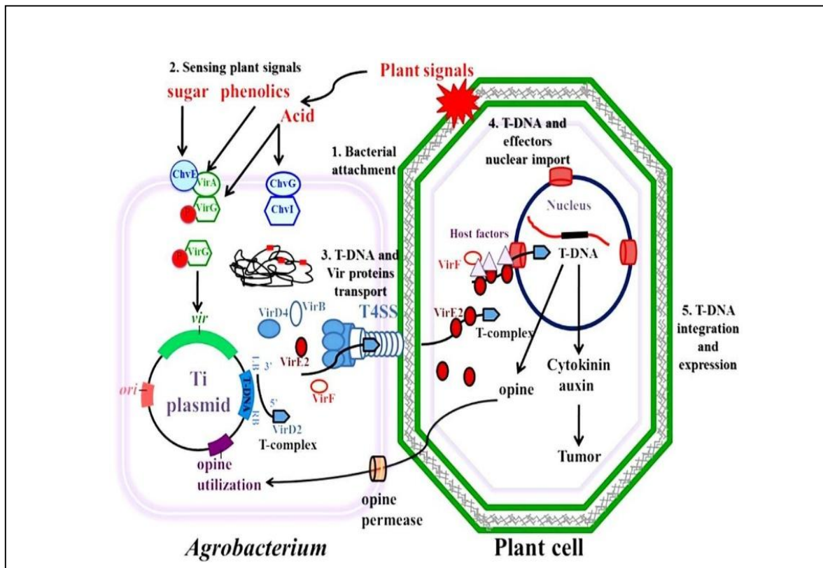
Figure2: Major steps of the A. tumefaciens mediated plant transformation process Source: The Arabidopsis book, 2017; BioOne
