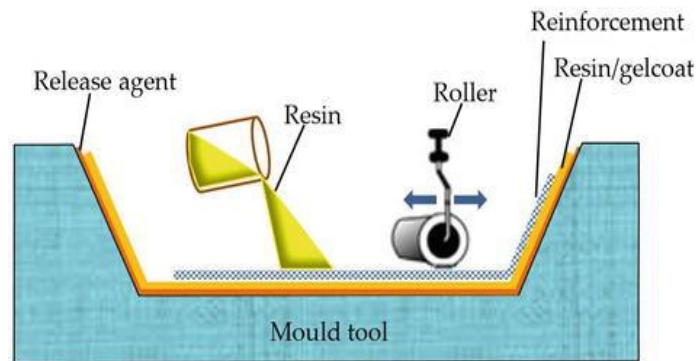
Figure 4: Hand Lay-Up [22]
