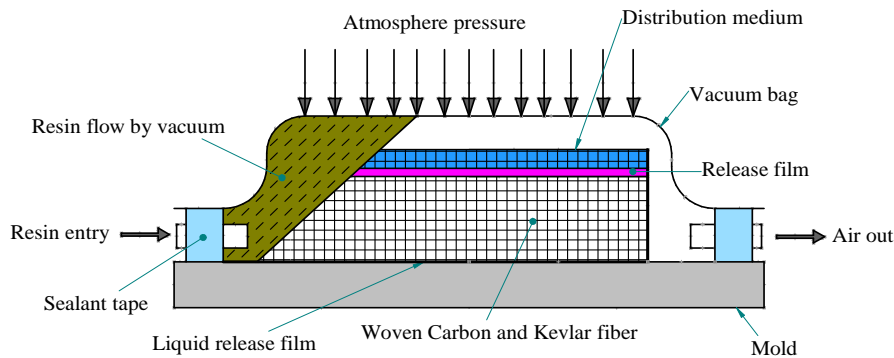
Figure 5: VARIM Method
