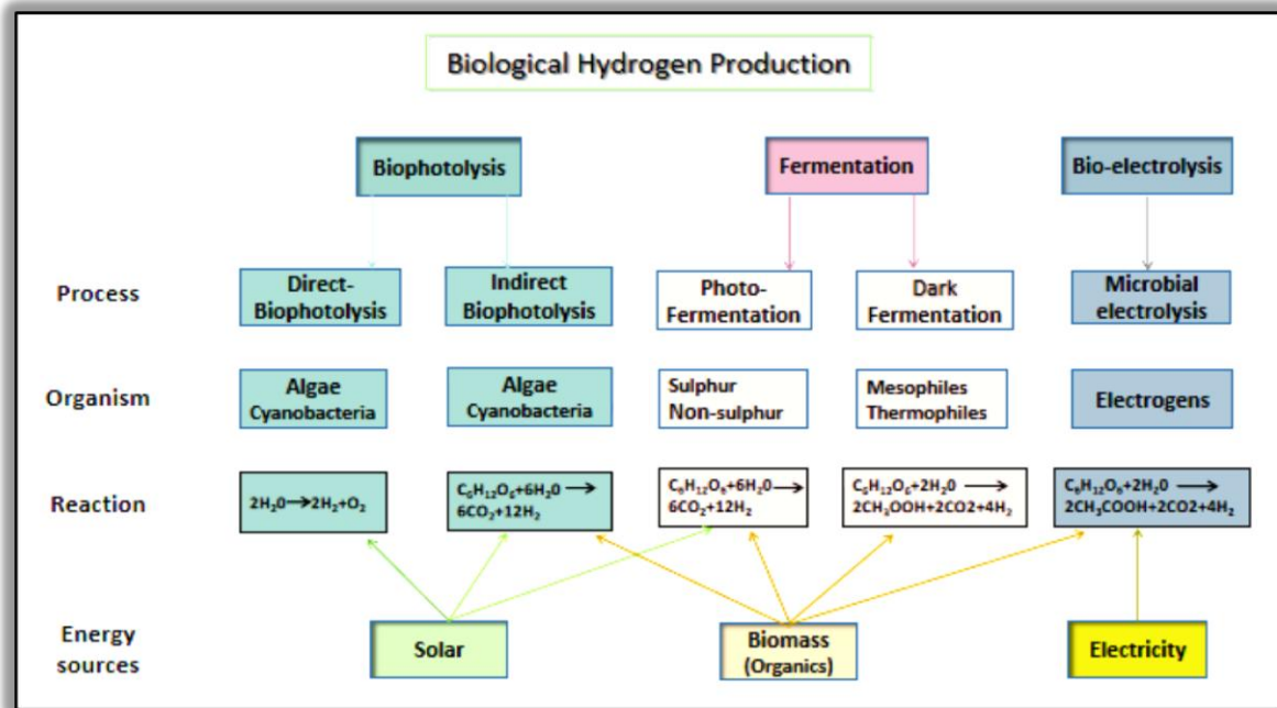
Figure 4: Methods for production of biological hydrogen
