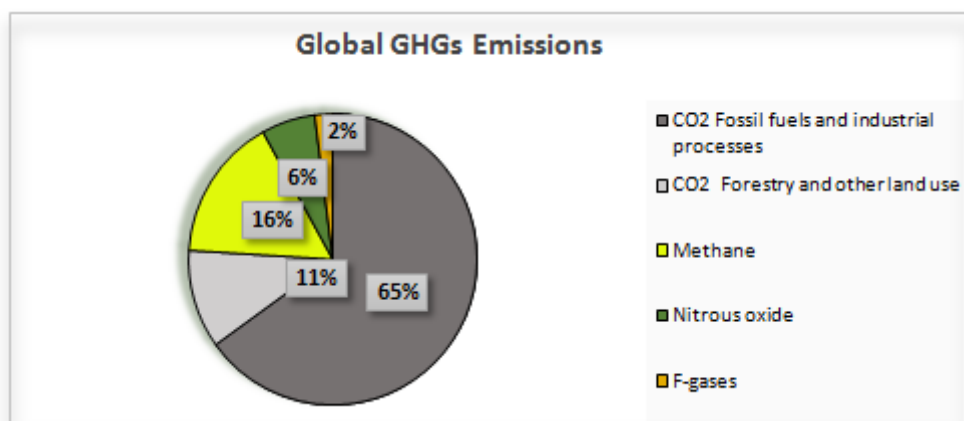
Figure 1: Global warming impact of GHGs
