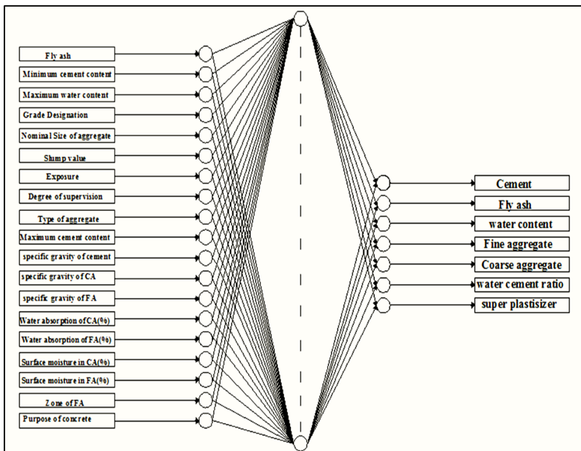
Figure 2: Specific ANN Topology
