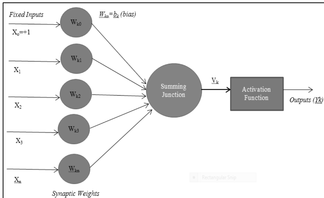
Figure 1: The General mathematical model of Artificial Neural Network
