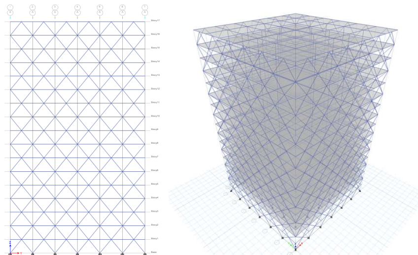
Figure 5: Elevation and 3D View of Diagrid Building with Diagrid Angle 52°
