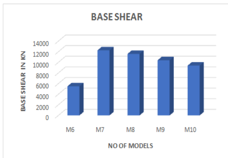
Graph 10: Base Shear in Kn for Model 6 to 10 Due to Seismic Load Along X and Y-Direction in Zone V
