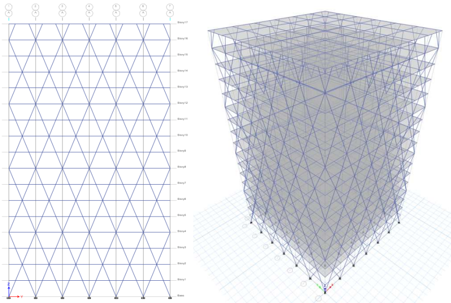
Figure 7: Elevation of Diagrid Building and 3D View of Diagrid Building with Diagrid Angle 68.66^\circ
