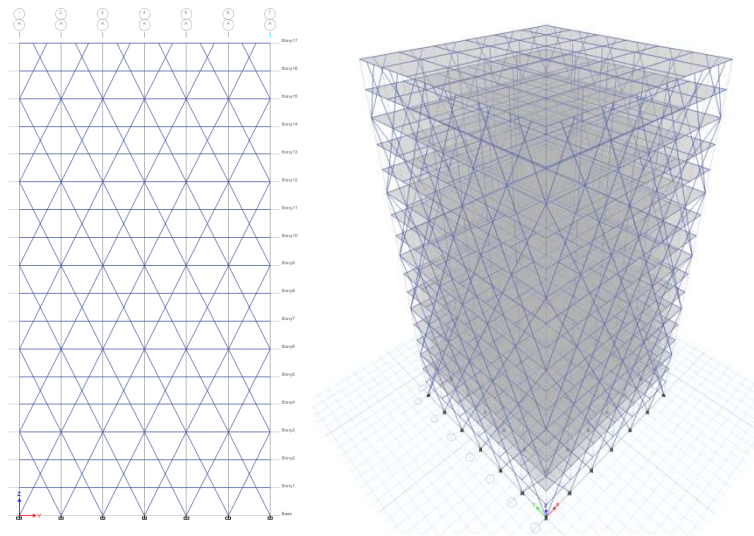
Figure 6: Elevation of Diagrid Building and 3D View of Diagrid Building with Diagrid Angle 62.48^\circ
