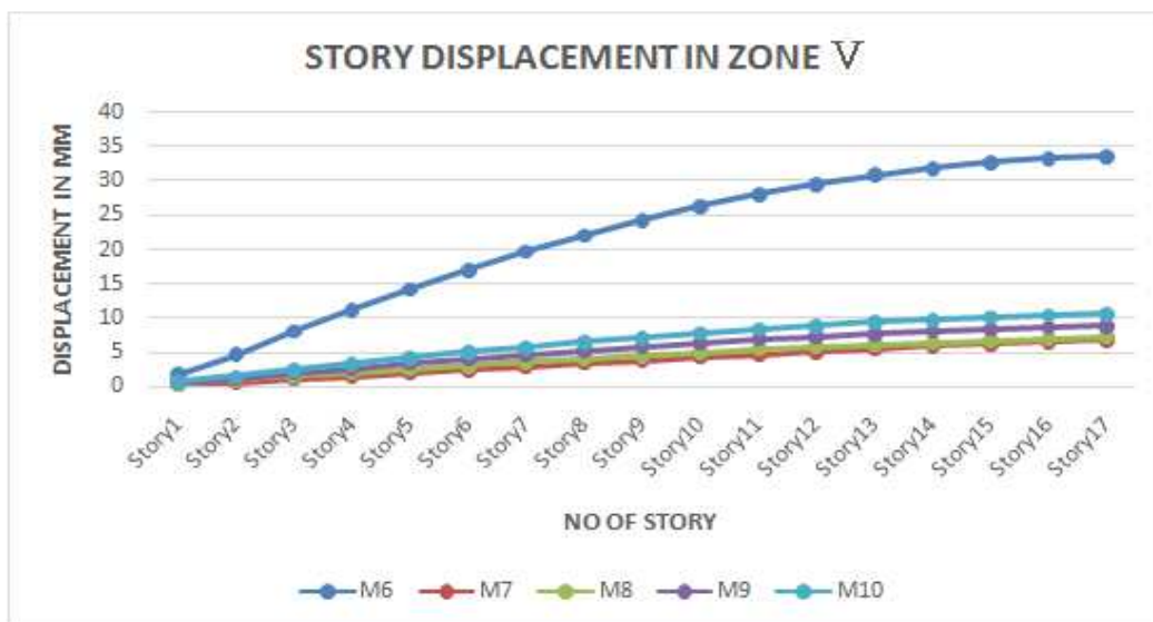
Graph 2: Story Displacement in Mm for Model 6 to 10 Due to Wind Load Along X & Y-Dir in Zone V
