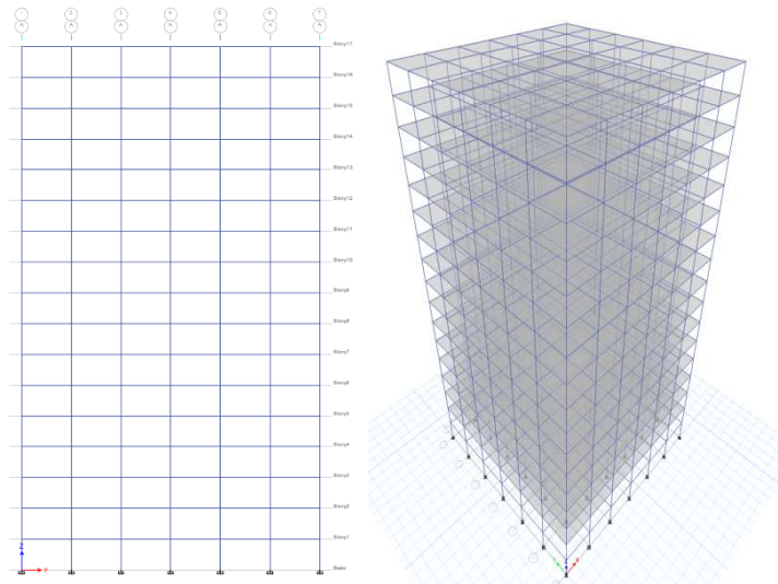
Figure 4: Elevation of and 3D View of RC Bare Frame Building
