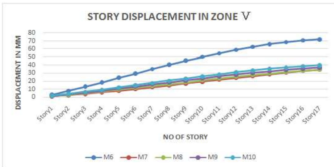
Graph 6: Story Displacement in Mm for Model 6 to 10 Due to Seismic Load Along X& Y- Dir in Zone V
