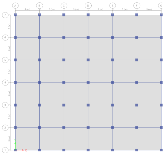
Figure 2: Plan of Multi-Story RC Bare Frame Building
