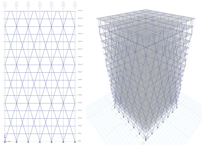
Figure 8: Elevation of Diagrid Building and 3D View of Diagrid Building with Diagrid Angle 72.64°
