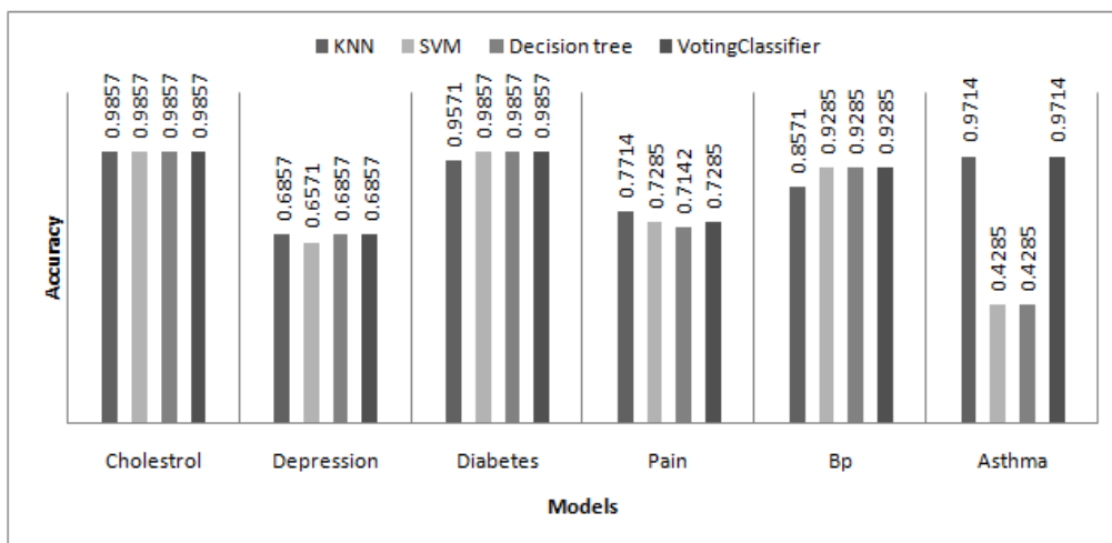
Figure 2: Drug type prediction accuracy comparisons chart
