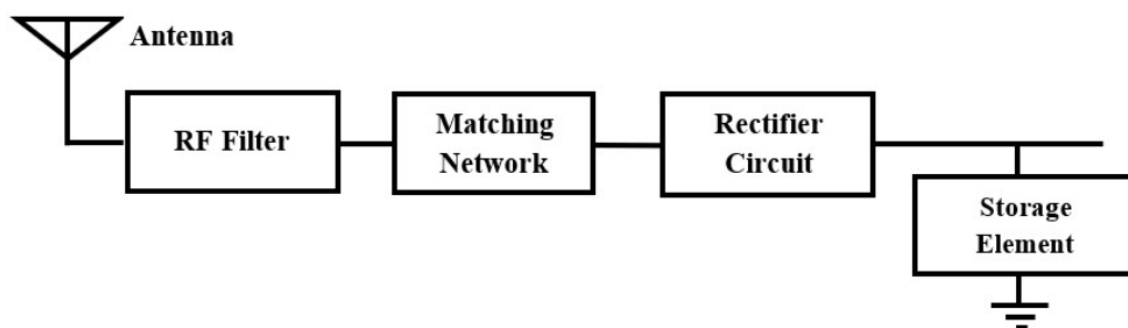
Figure 5: Block diagram of a Rectenna System [28].
