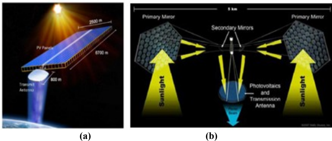
Figure 8: (a) Solar Power Satellite System [9], [b] Photovoltaic Cells [9].
