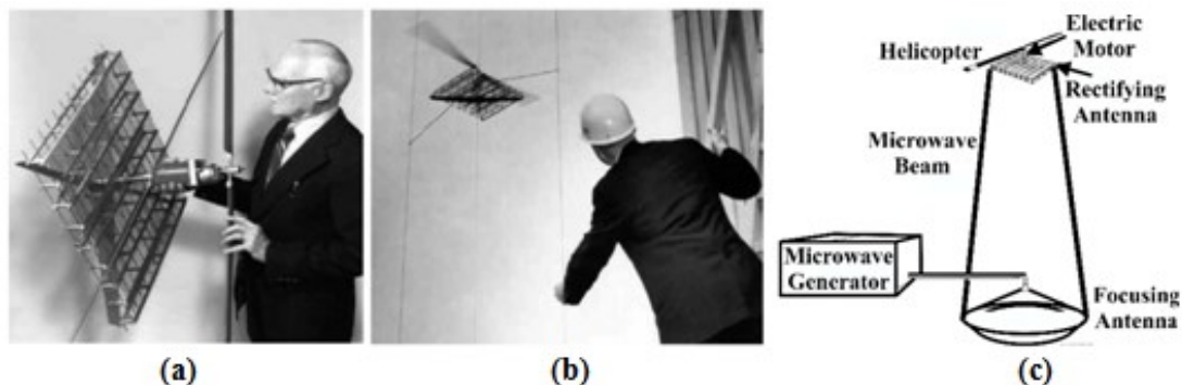
Figure 7: (a) Close-up view of the Microwave-Powered Helicopter, (b) View of the Helicopter in Flight at an Altitude of 30 ft [32], (c) Basic Design Elements of the Microwave-Powered Helicopter [33].
