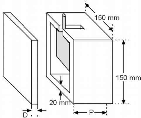
Figure 13: Rectenna System Embedded in Buried Concrete [42].
