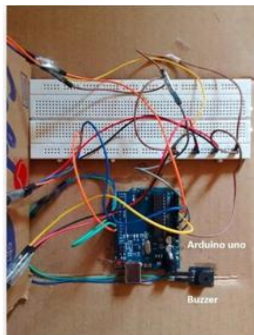
Figure 5: The Connection of Arduino uno and the buzzer
