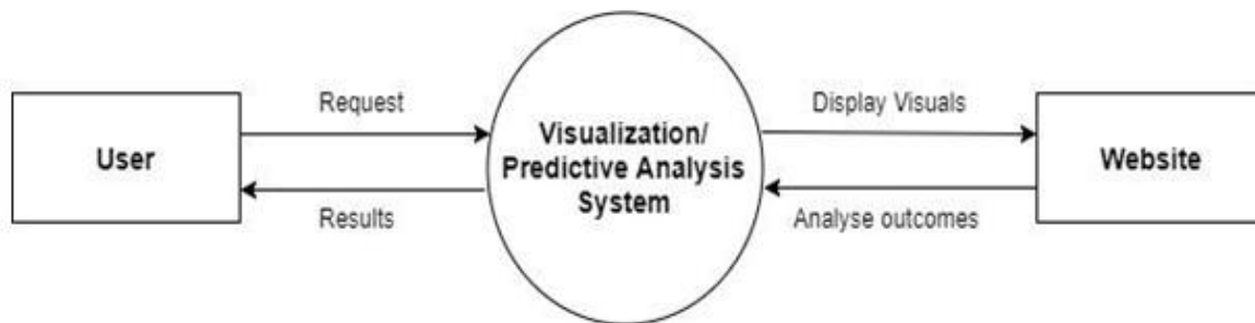
Figure 1: Architectural DFD
