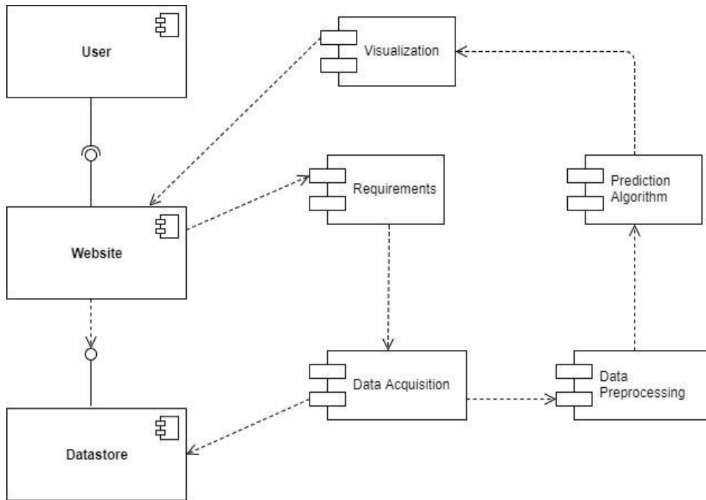
Figure 3: Component Diagram
