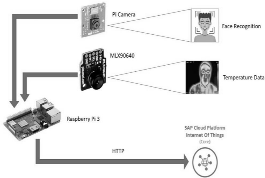
Figure 1.5: Application of IoT Enabled Thermal Camera
