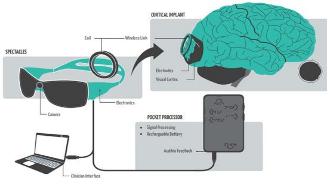
Figure 4: Image shows an overview of MVG cortical visual prosthesis
