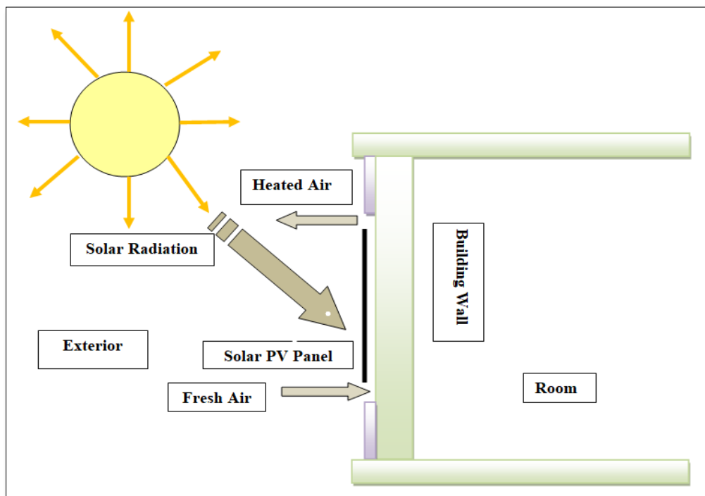
Figure 1: Schematic Diagram of BIPV (Adapted from Debbarma, et. al., 2017).
