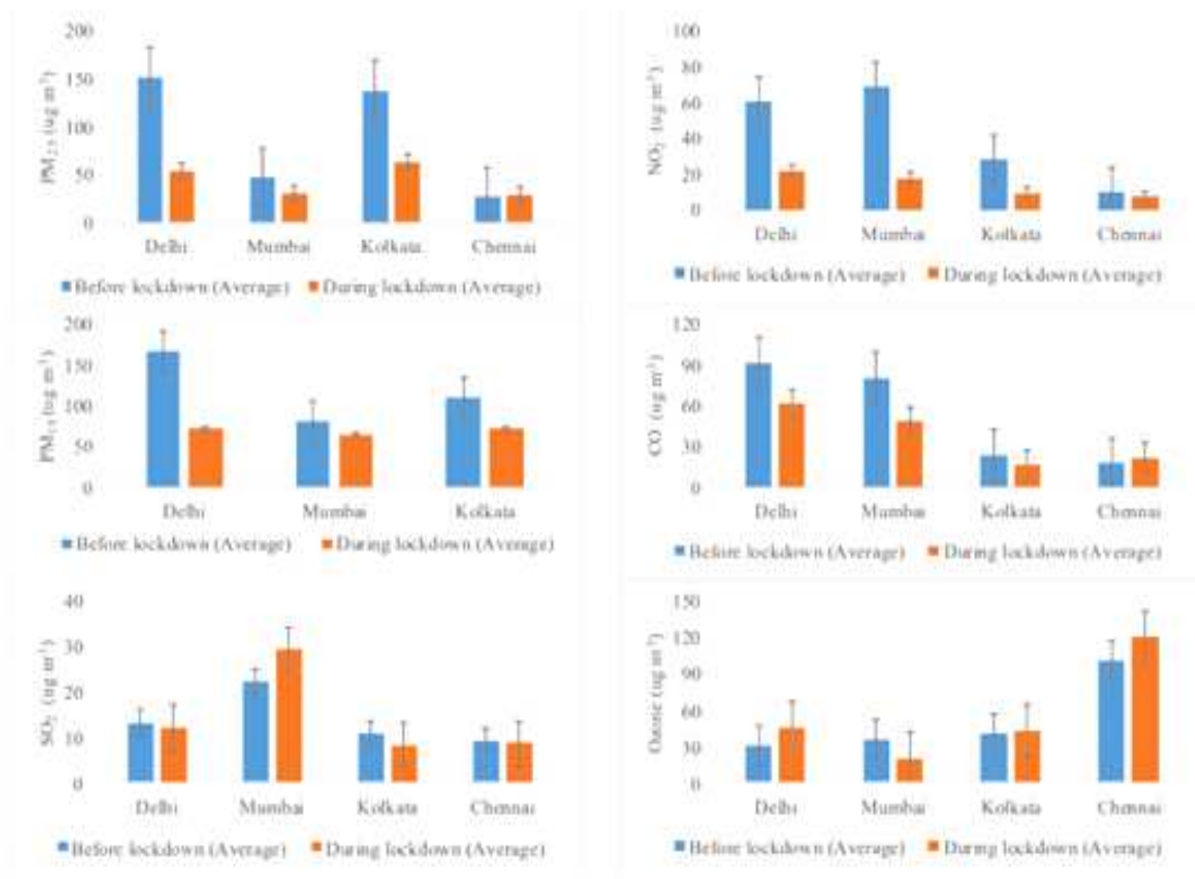
Figure 4: Pollution levels before and during lockdown - Indian cities
