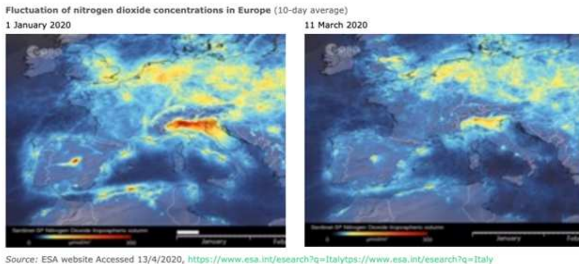
Figure 2: Nitrogen dioxide concentration
