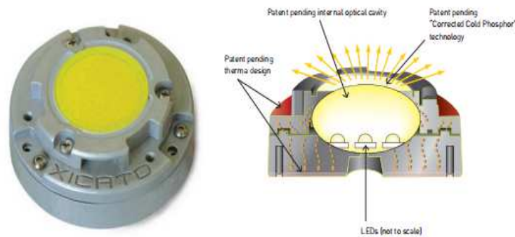
Figure 17: Left: An LED light; Right: This drawing, by the manufacturer, shows a section through an Xicato white LED module. [Source: Lighting for Interior Design]
