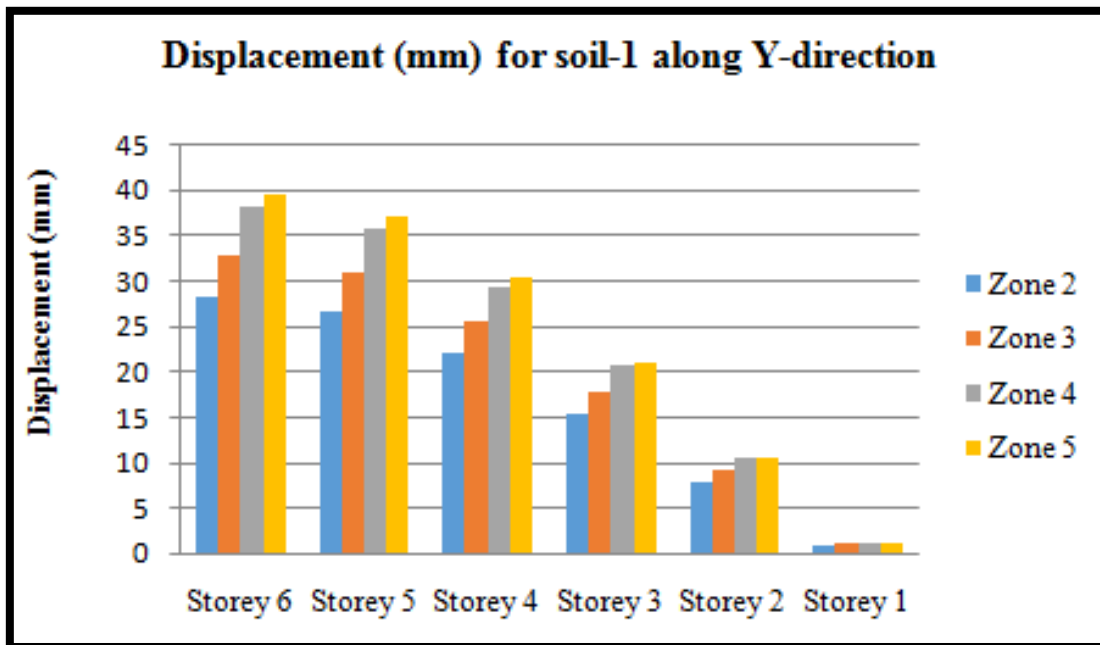
Figure 9: Displacement (mm) for soil-1 along Y-direction
