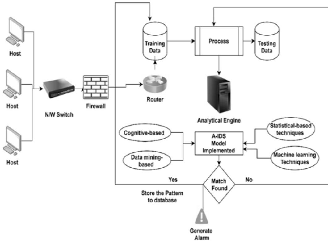
Figure 3: Anomaly Intrusion Detection System Working Process
