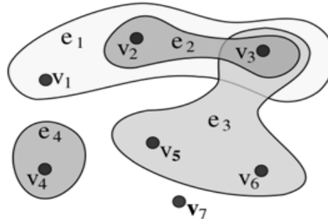
Figure 4: Hypergraph
