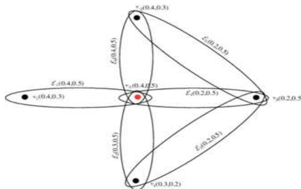
Figure 9: Intuitionistic Fuzzy Threshold Graph
