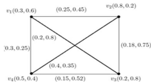
Figure 5: Intuitionistic Fuzzy Graph
