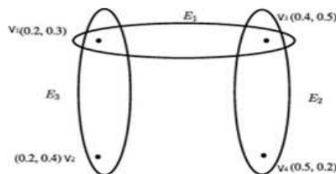
Figure 8: Intuitionistic Fuzzy Hypergraph
