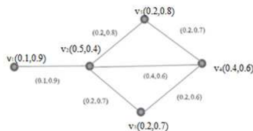
Figure 7: Intuitionistic Fuzzy Threshold Graph
