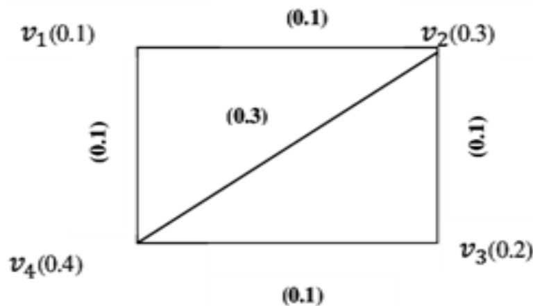
Figure 4: Fuzzy Graph
