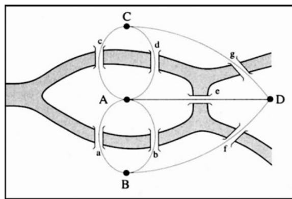
Figure 1: Seven Bridges of Königsberg
