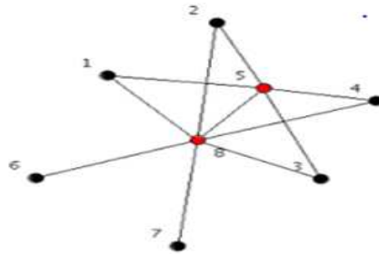
Figure 6: Threshold graph
