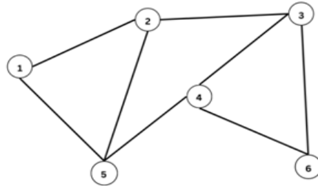
Figure 3: Undirected graph
