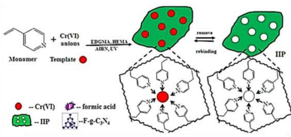
Figure 10: Schematic illustration of the formation process of the IIP [77].
