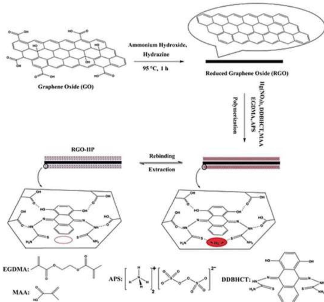
Figure 9: Preparation of reduced graphene oxide-ion-imprinted polymer modified glassy carbon electrode [77].
