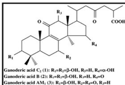
Figure 2: Chemical Structure of some Ganoderic Acids
