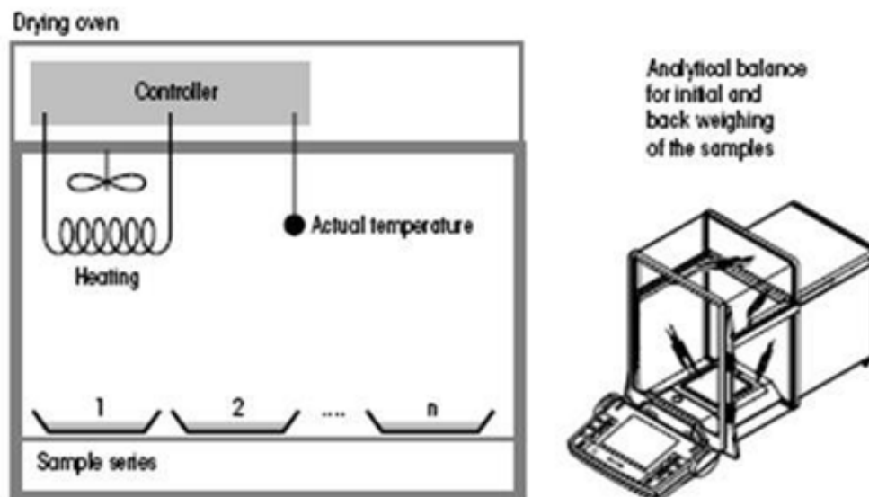
Figure 1: Thermo-Gravimetric Technique of Soil Measurement [5]
