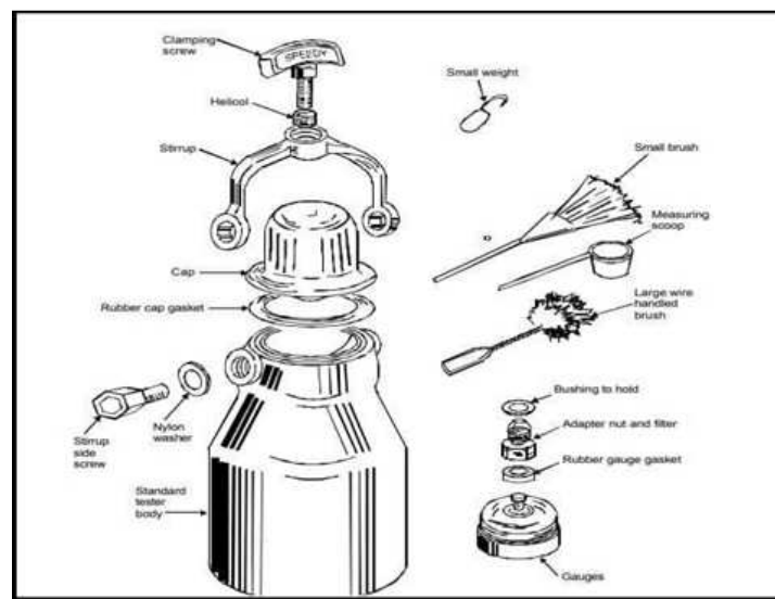
Figure 2: Calcium Carbide Tester [5]
