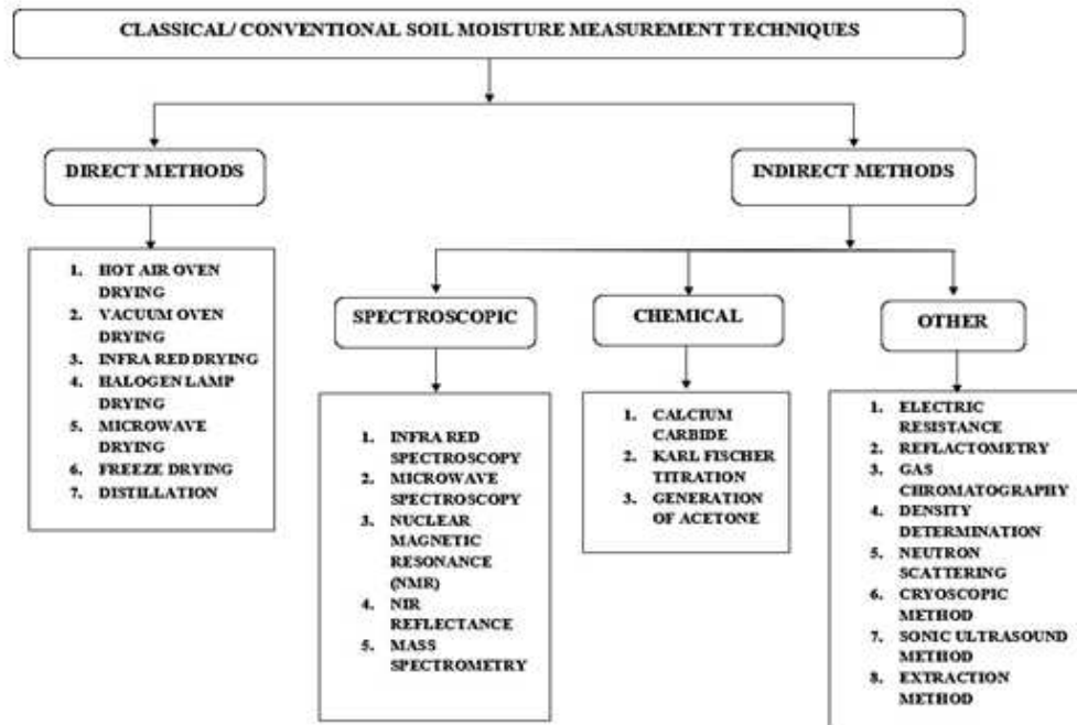
Figure 3: Classical/ Conventional Soil- Moisture Sensing Techniques
