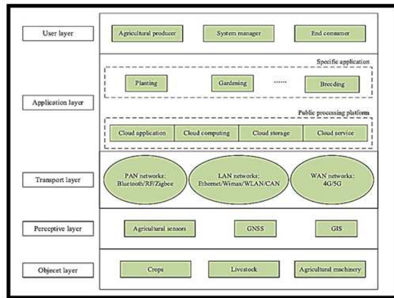
Figure 2: Architecture of Agricultural IoT [12]
