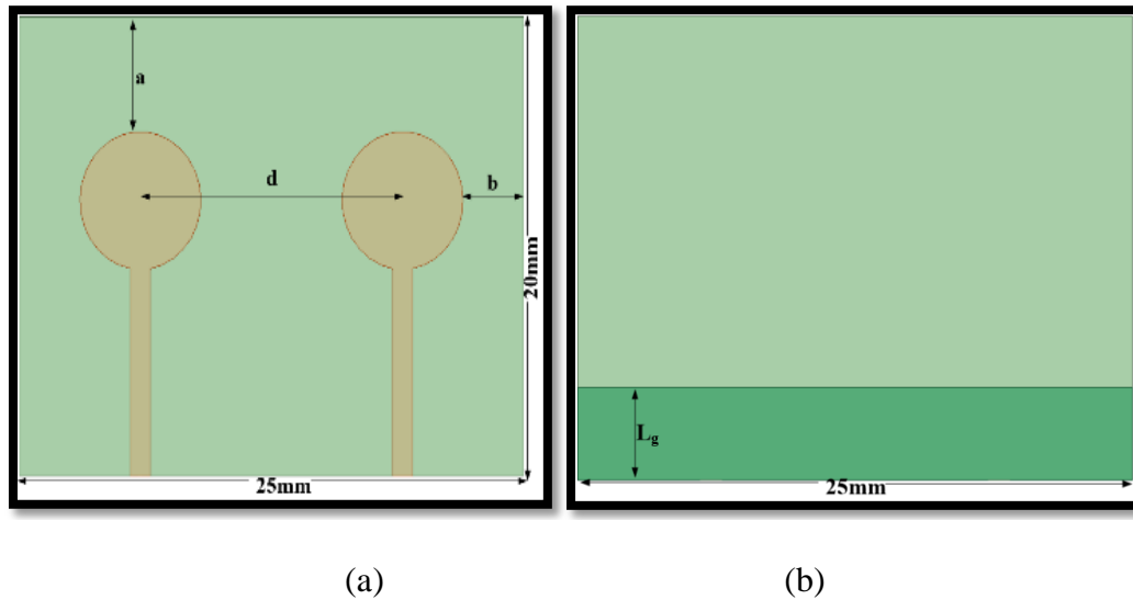
Figure 3: MIMO antenna (a) Front view, (b) Back view, d=13\text{mm} ( 0.9\lambda_0 ), a=5\text{mm} , b=3\text{mm}
