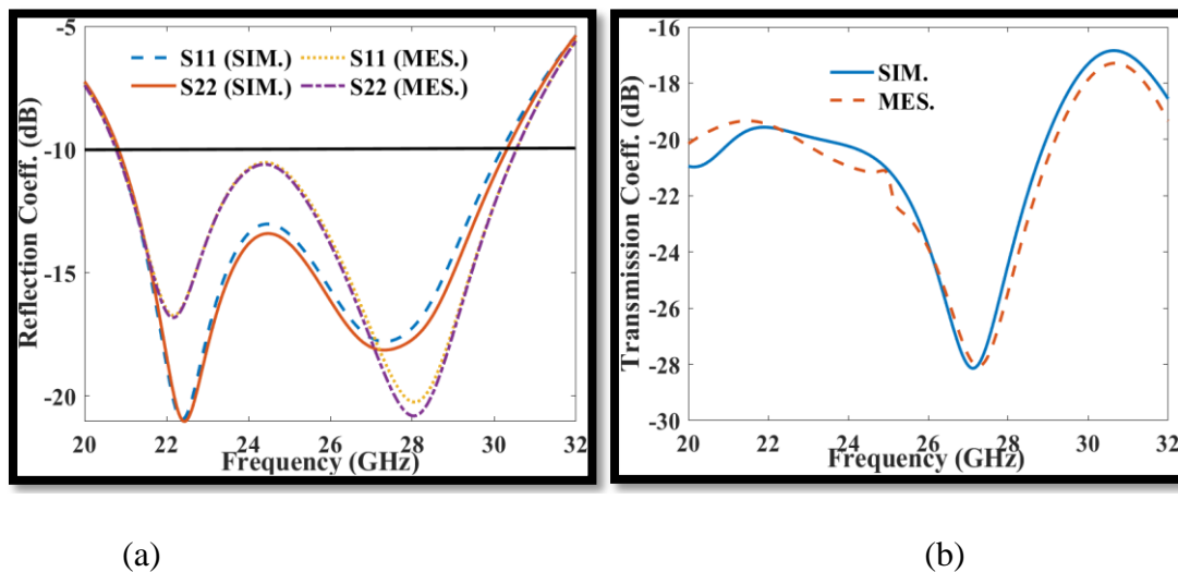
Figure 4: (a) Reflection coefficient (S11) (b) Transmission coefficient (S12)
