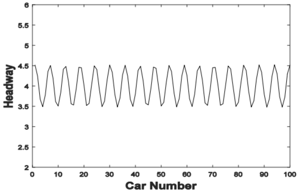
Figure 26: Headway profiles at t = 10000 s, for \lambda = 0.5 and p = 0.2
