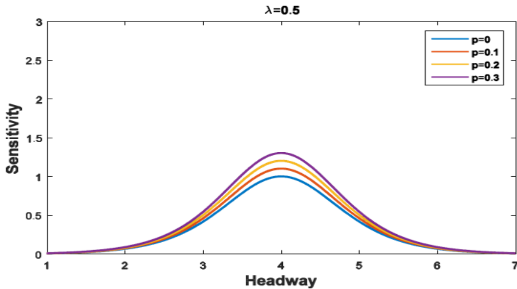
Figure 3: Neutral stability curves in the headway-sensitivity space for \lambda = 0.5 and distinct values of p .
