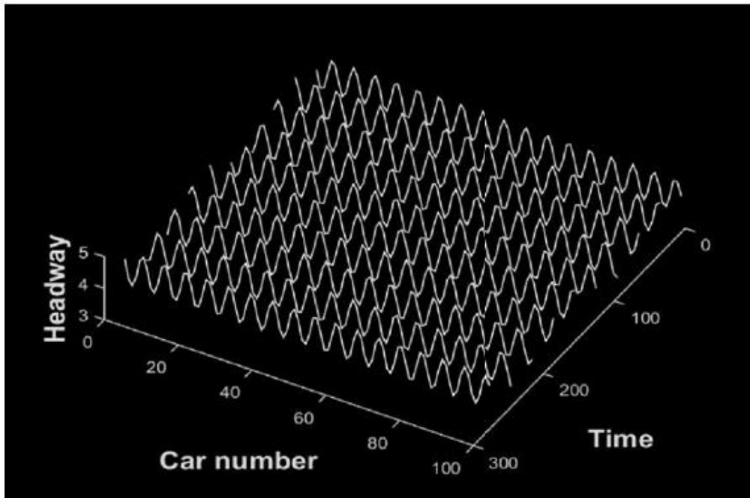
Figure 22: Headway evolution in space and time after t = 10000s for \lambda = 0.5 and p = 0.2 .
