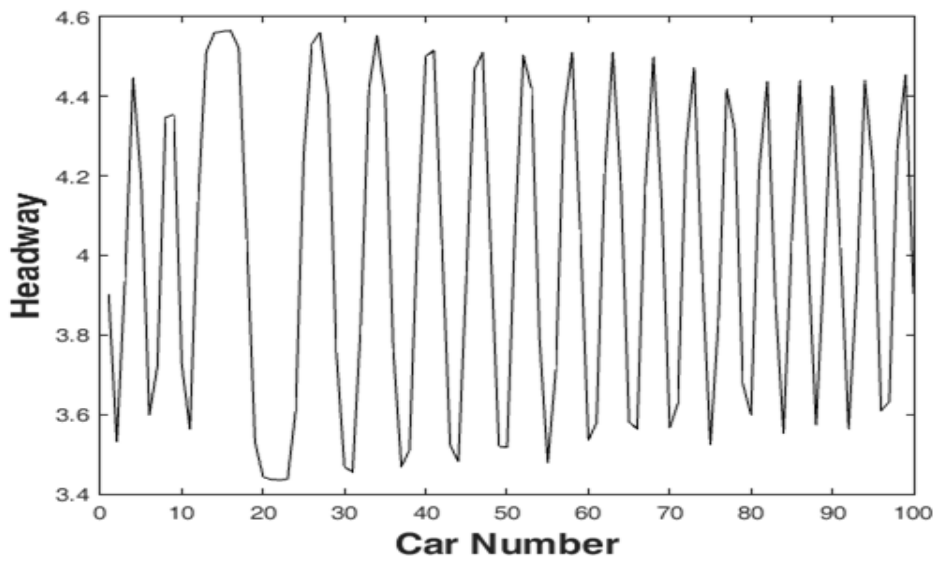
Figure 10: Headway profiles at t=10000s , for \lambda = 0 and p = 0.2
