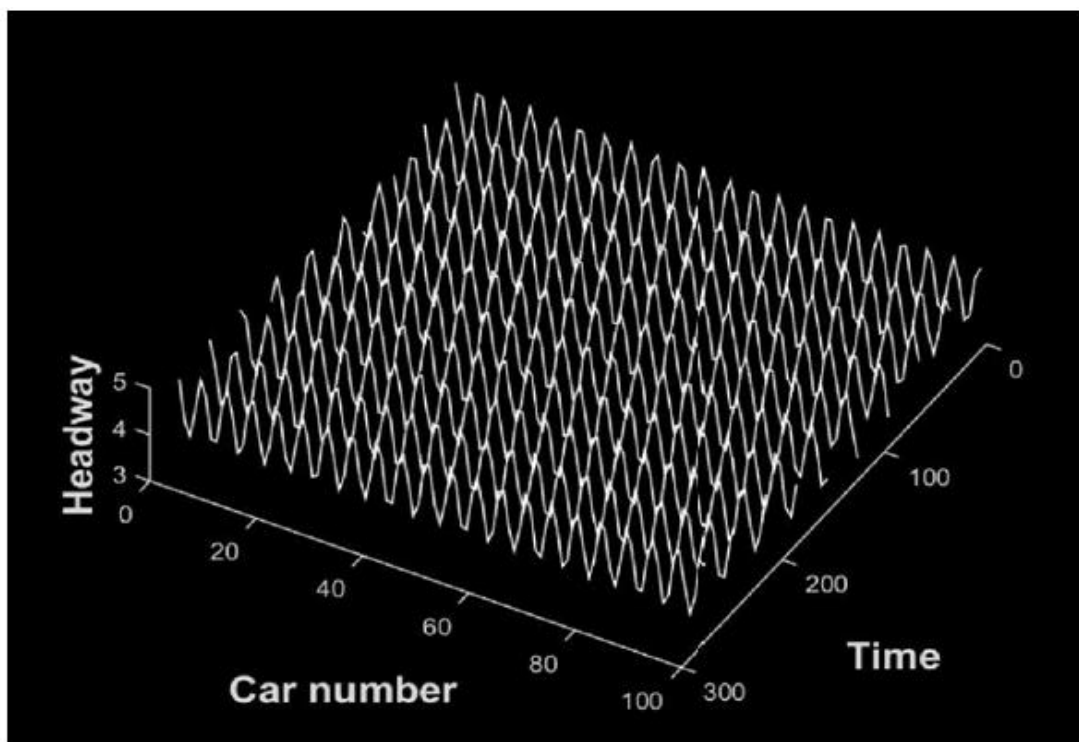
Figure 23: Headway evolution in space and time after t = 10000s for \lambda = 0.5 and p = 0.3 .
