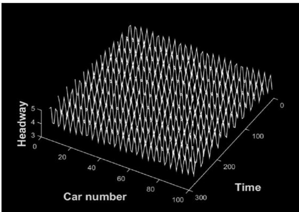
Figure 15: Headway evolution in space and time after t = 10000s for \lambda = 0.3 and p = 0.3
