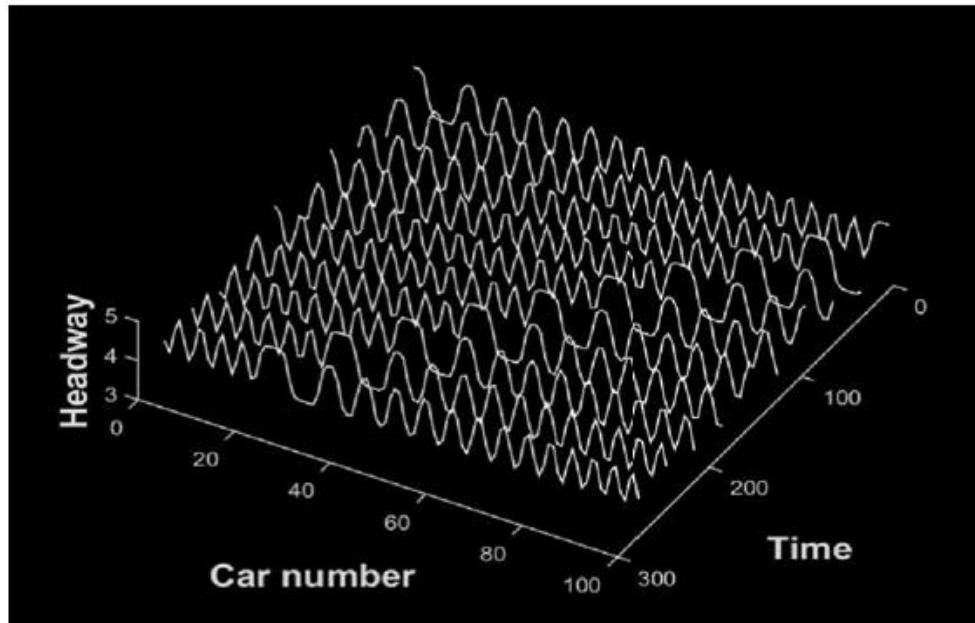
Figure 5: Headway evolution in space and time after t = 10000s for \lambda = 0 and p = 0.1
