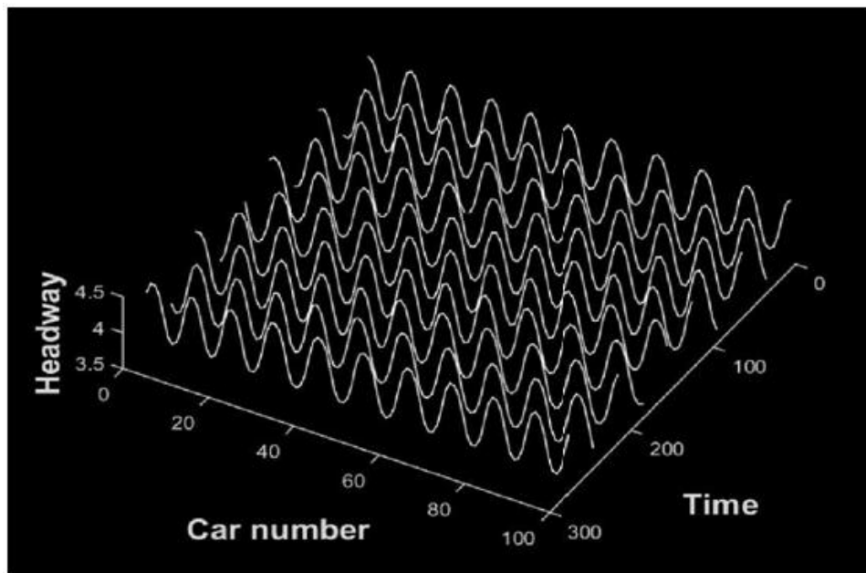
Figure 13: Headway evolution in space and time after t = 10000s for \lambda = 0.3 and p = 0.1 .
