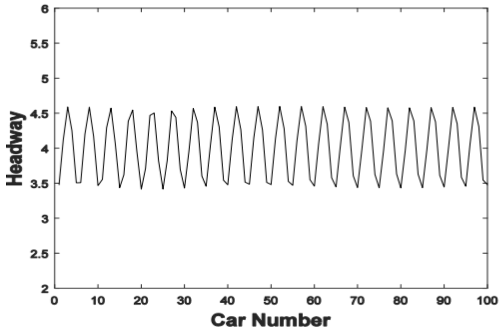
Figure 18: Headway profiles at t = 10000 s, for \lambda = 0.3 and p = 0.2
