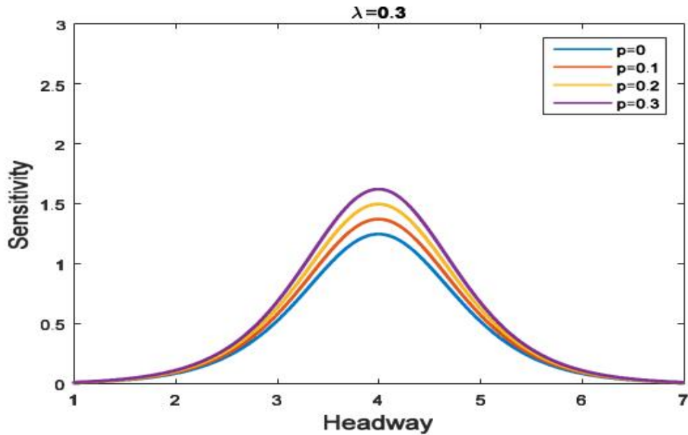
Figure 2: Neutral stability curves in the headway-sensitivity space for \lambda = 0.3 and distinct values of p .
