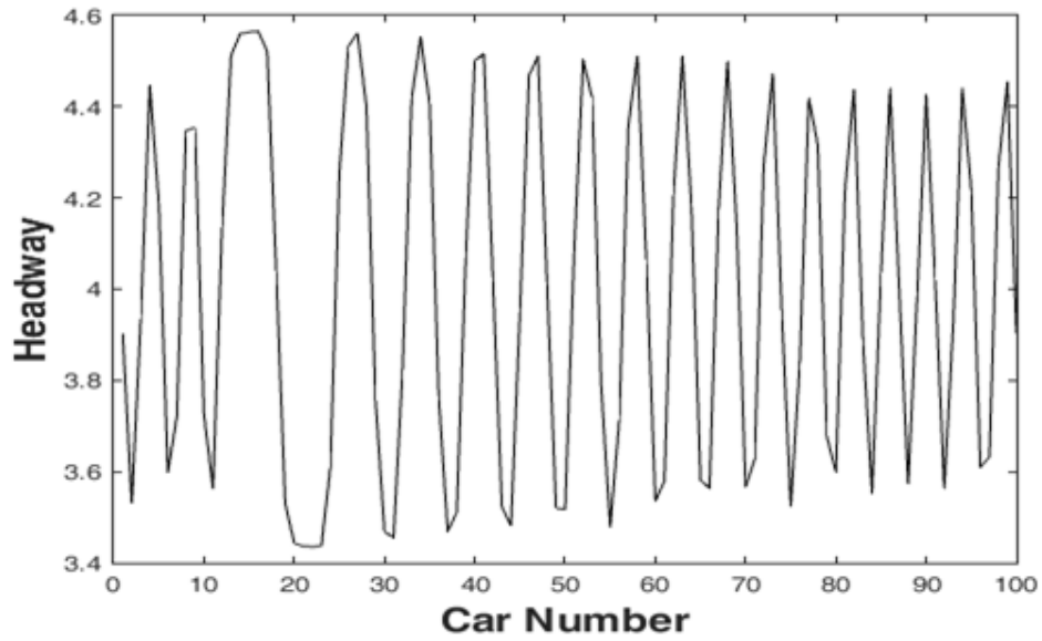
Figure 9: Headway profiles at t=10000s , for \lambda = 0 and p = 0.1
