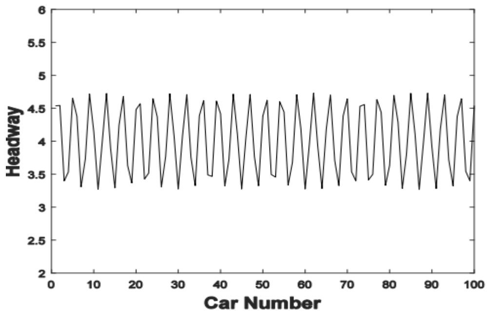
Figure 19: Headway profiles at t = 10000 s, for \lambda = 0.3 and p = 0.3
