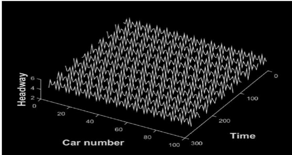
Figure 7: Headway evolution in space and time after t = 10000s for \lambda = 0 and p = 0.3
