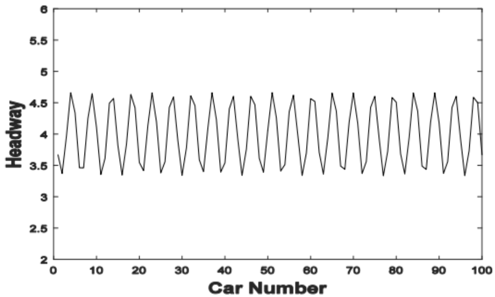
Figure 27: Headway profiles at t = 10000 s, for \lambda = 0.5 and p = 0.3
