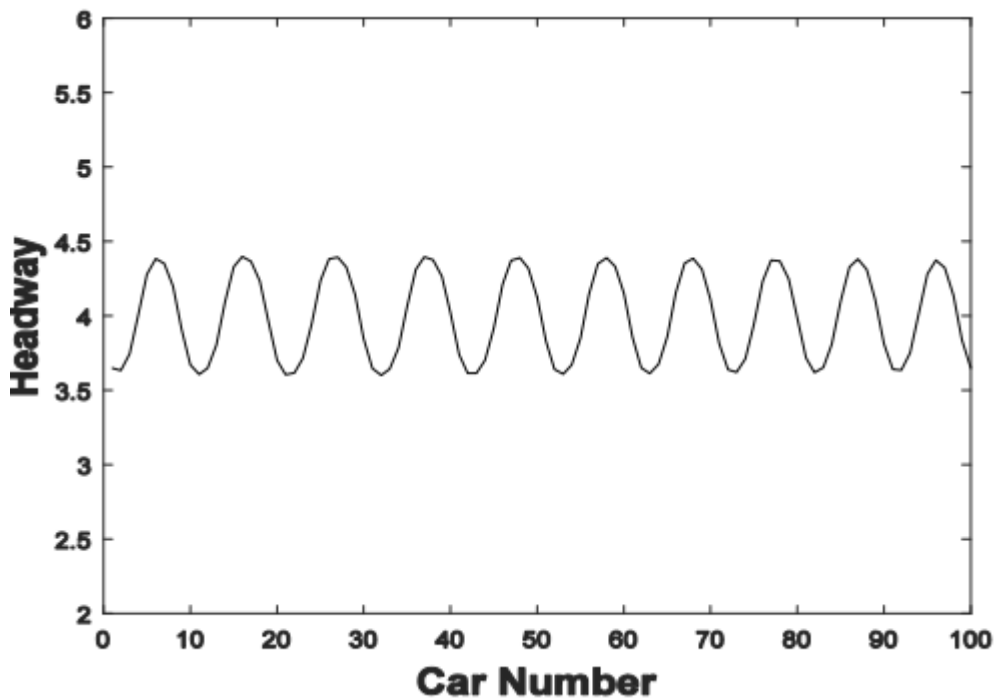
Figure 17: Headway profiles at t=10000s , for \lambda = 0.3 and p = 0.1
