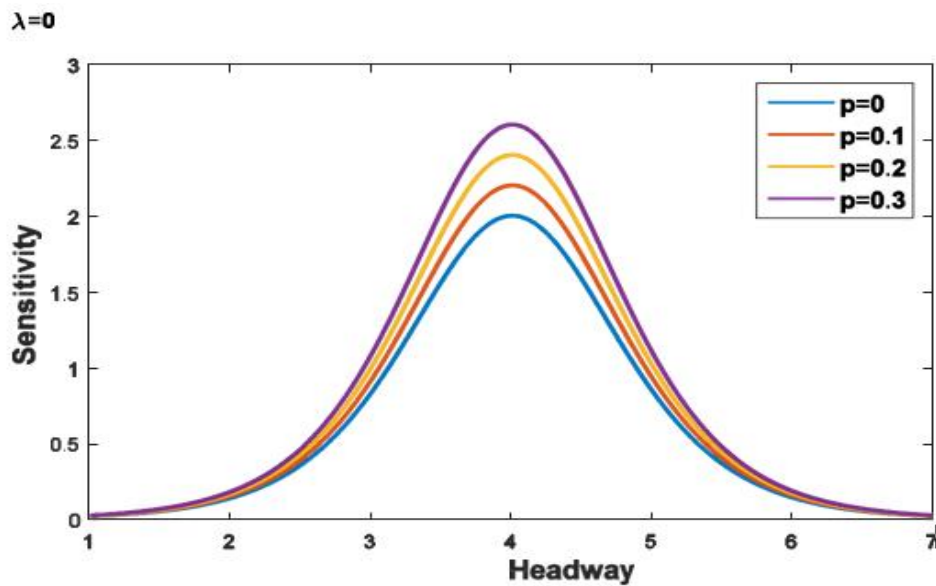
Figure 1: Neutral Stability Curves in the headway-sensitivity Space for \lambda = 0 and distinct Values of p
