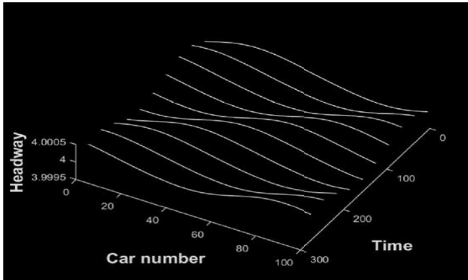
Figure 12: Headway evolution in space and time after t = 10000s for \lambda = 0.3 and p = 0 .
