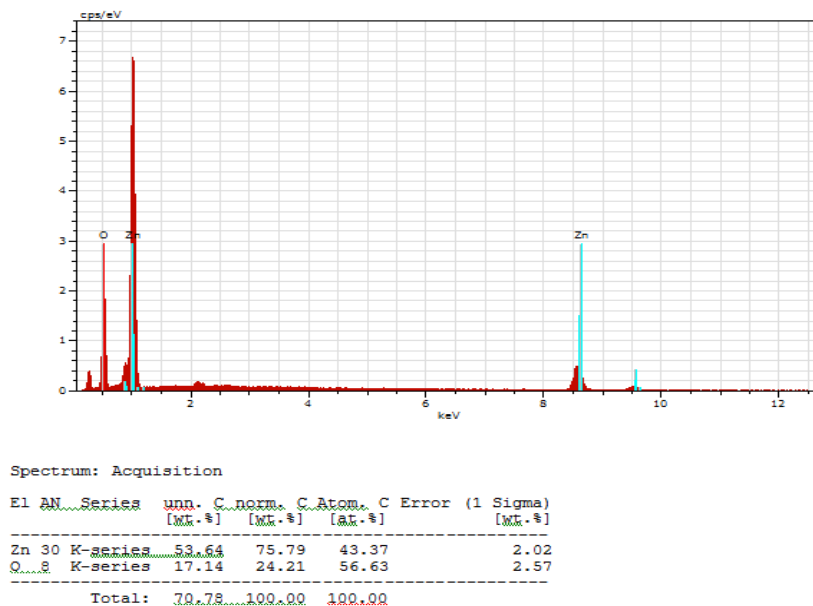
Figure 7: EDX analysis of the ZnO nanoparticles prepared through green
