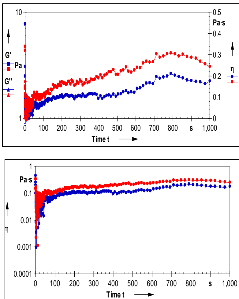
Figure 9: Rheological parameters calculated using the Rheometer a) Shear strain vs frequency graph b) G' and G'' vs time graph c) Viscosity ( \eta ) vs time graph.
