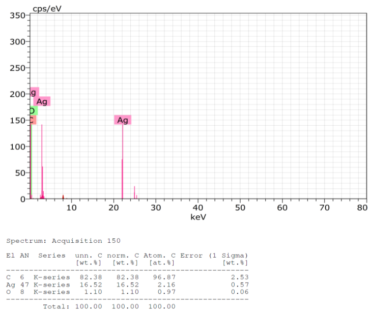
Figure 4: EDX results for AgNPs-PVA nanocomposites
