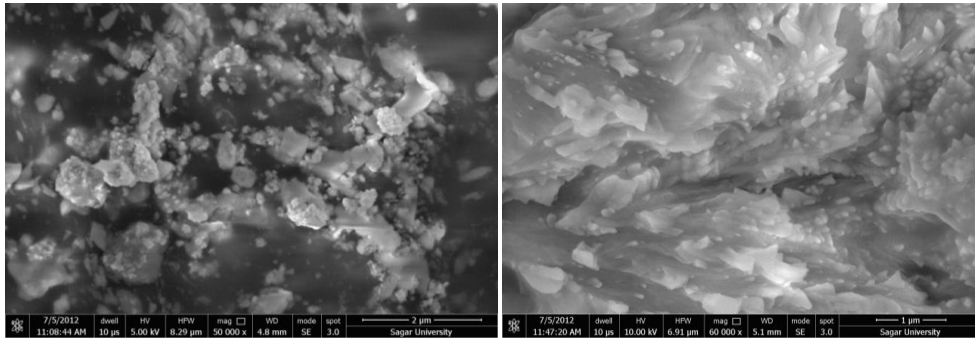
Figure 5: SEM images for Cu NPs prepared using Green synthesis
