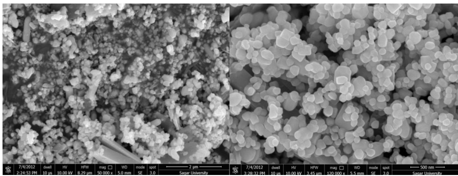
Figure 6: SEM images for ZnO nanoparticles prepared via Green synthesis
