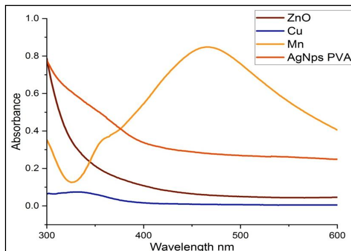
Figure 1: UV Visible spectroscopy of ZnO, Cu, Mn, and Ag-PVA nanoparticles in the range of 300-600nm
