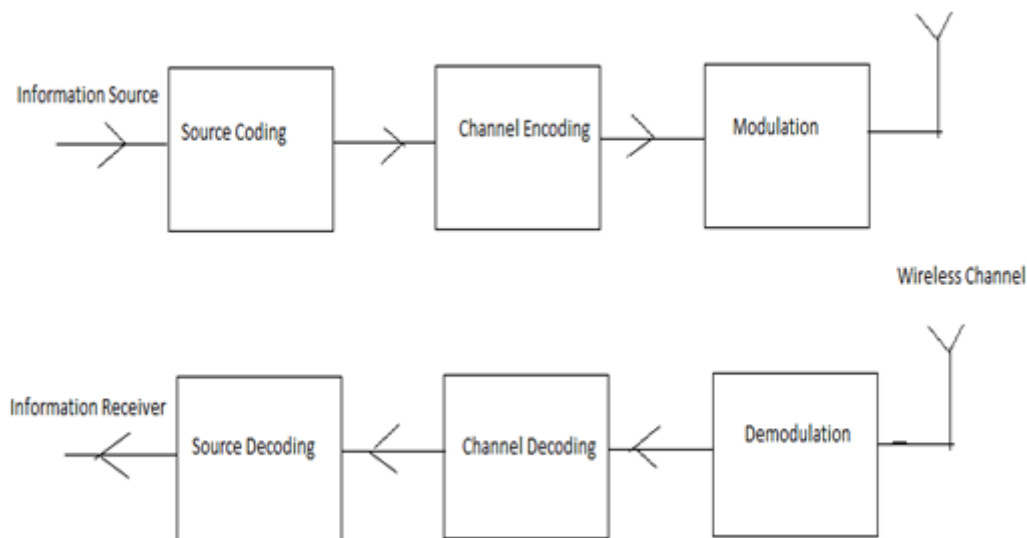
Figure 1: Block diagram of wireless communication system Key Components of Wireless
