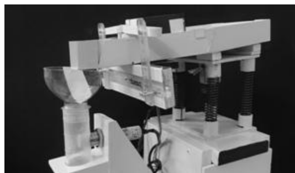
Figure 10: Vibrating Platform and feeder
