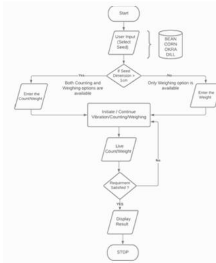
Figure 15: Flow Chart depicting the algorithm for seed quantification
