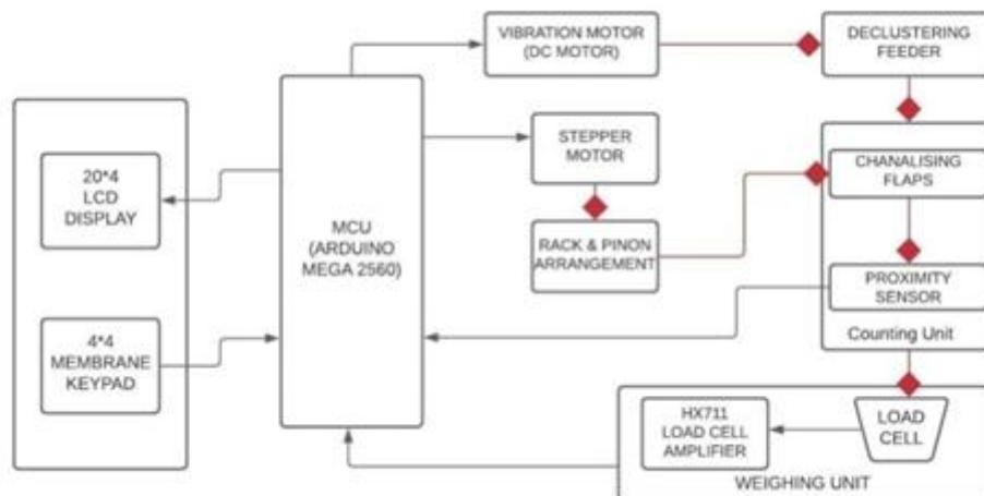
Figure 14: Block Diagram
