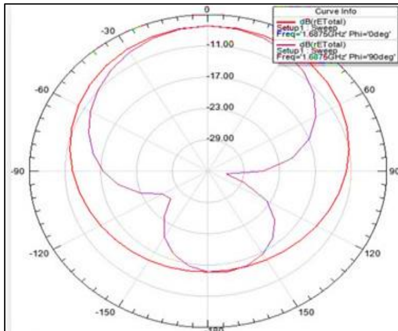
Figure 4: Radiation pattern of SQMSA at 2.38 GHz
