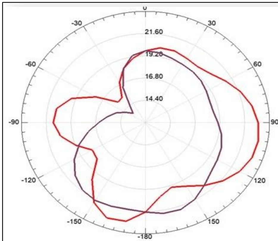
Figure 7: Radiation pattern of SQMSA at 4.83 GHz
