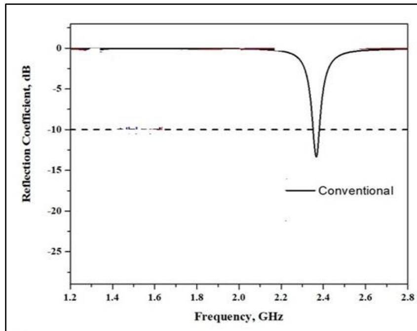
Figure 3: Measured return loss characteristics of 2.4GHz SQMSA
