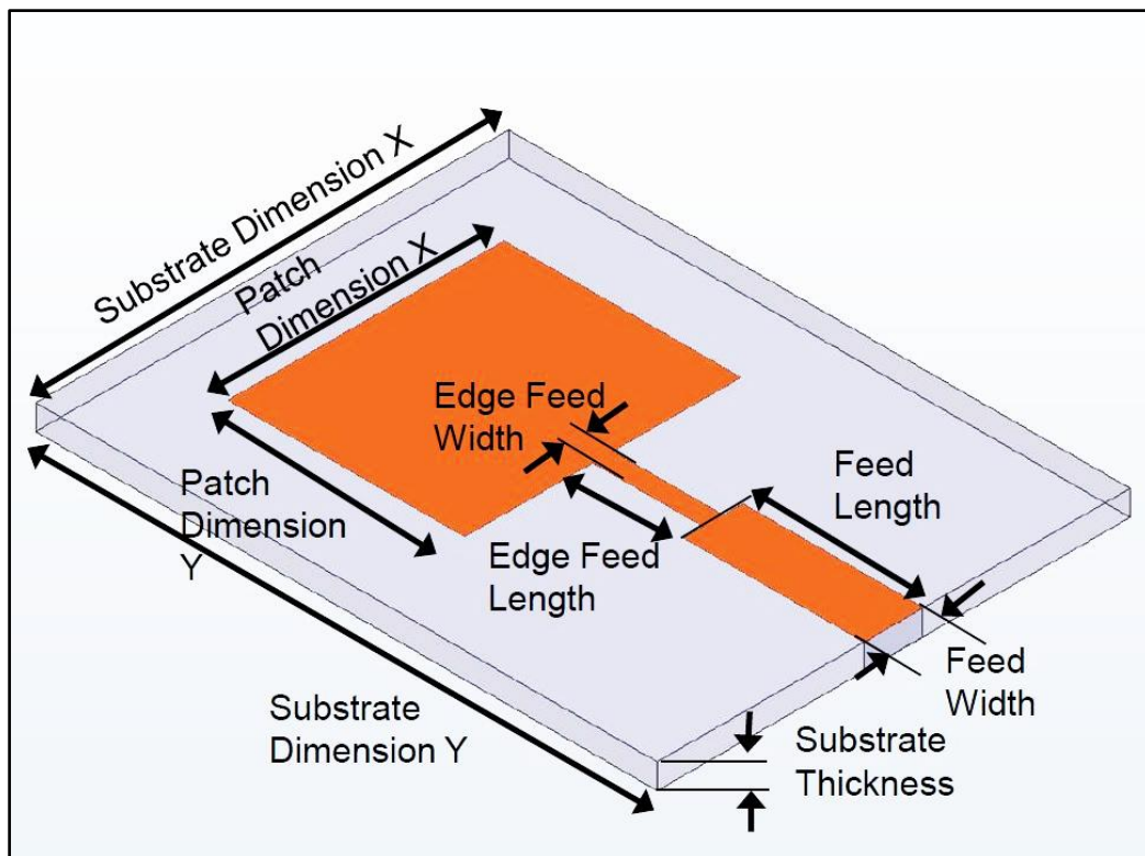
Figure 1: Geometry of SQMSA
