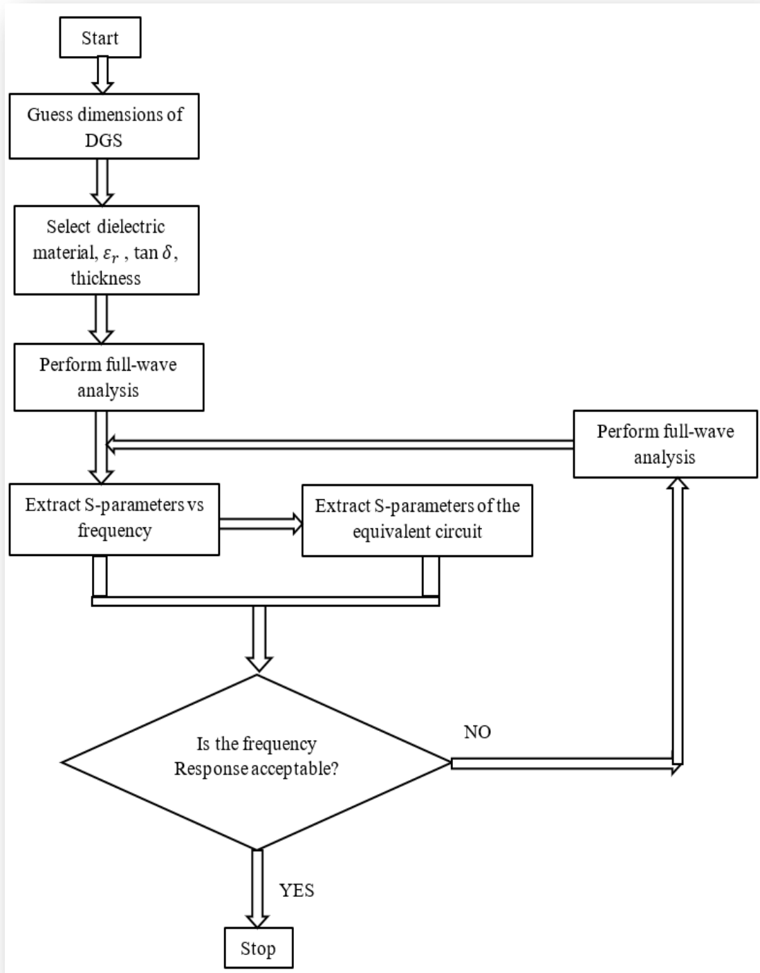
Figure 8: Conventional design and analysis method of dumbbell DGS.
