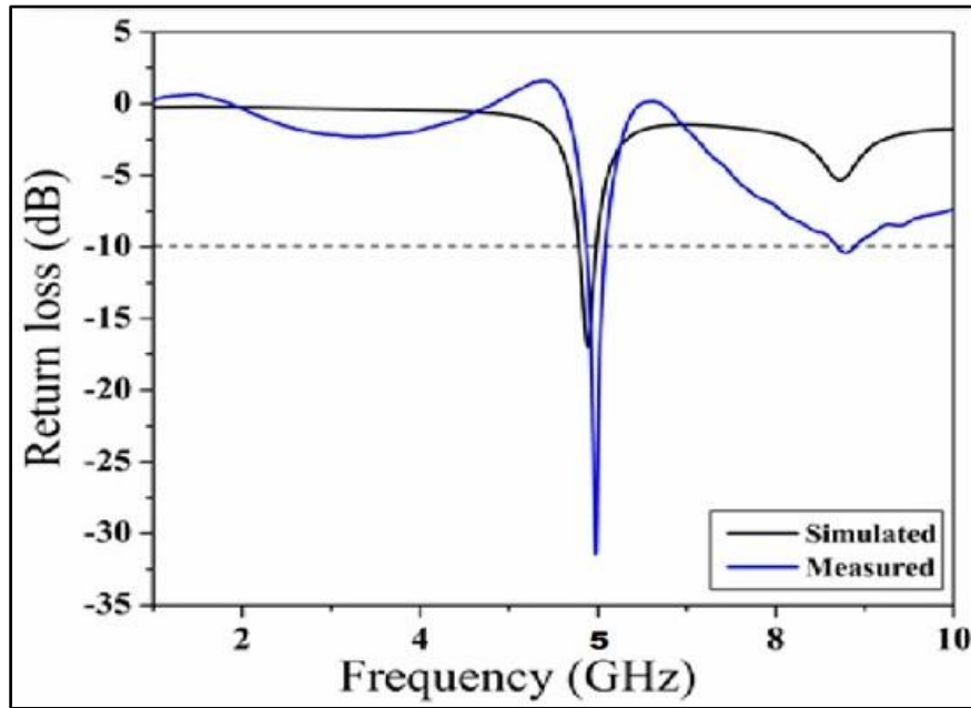
Figure 6: Simulated and measured return loss characteristics of SQMSA
