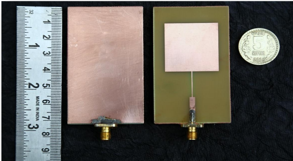
(b) Photographic view of the conventional 2.4 GHz SQMSA
