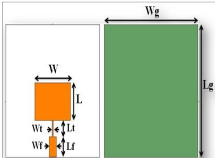
(a) Design Geometry
