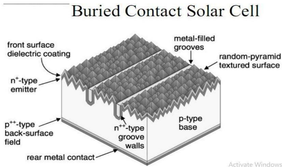
Figure 2: Buried contact solar cell
