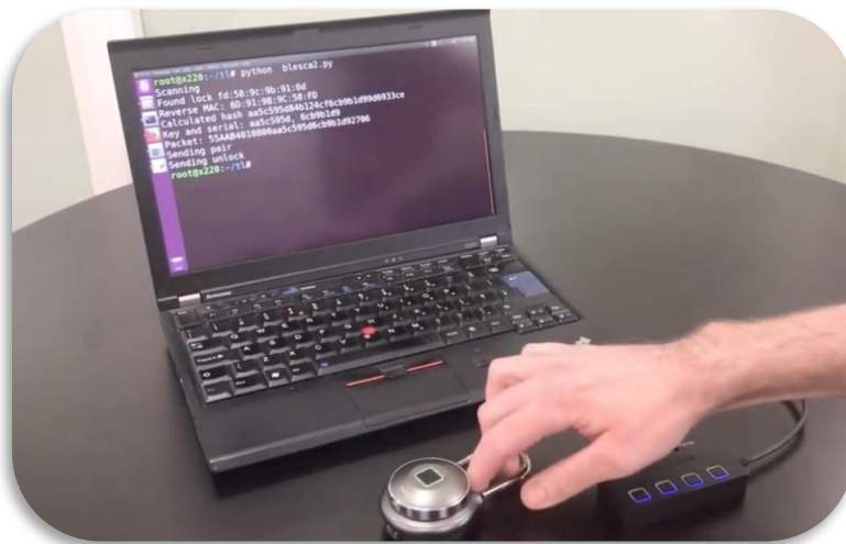
Figure 1: Tapp Padlock [1]
