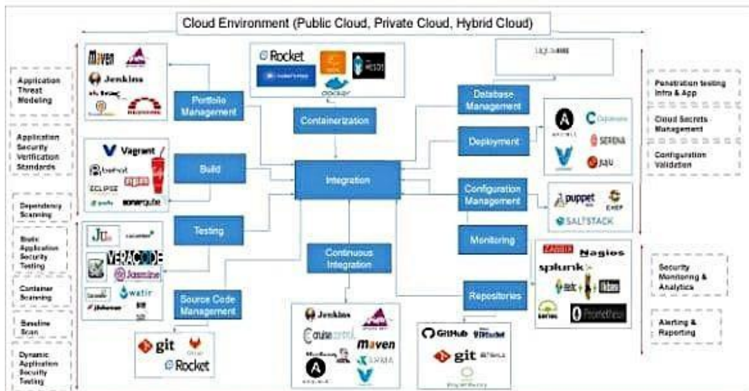
Figure 1: DevSecOps lifecycle and open source tool mapping
