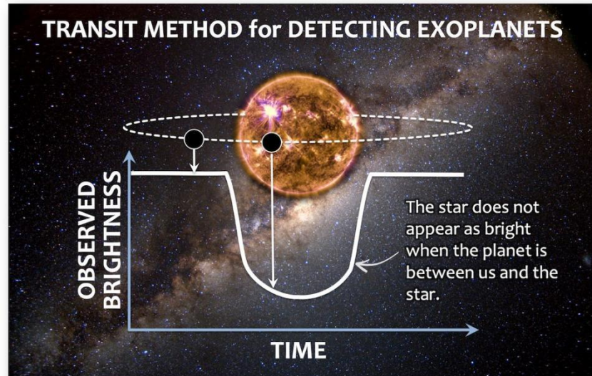
Figure 3: Transit Method: A schematic representation of the transit method used to detect exoplanets. The figure demonstrates how the periodic dimming of a star's light can indicate the presence of a planet passing in front of it.
