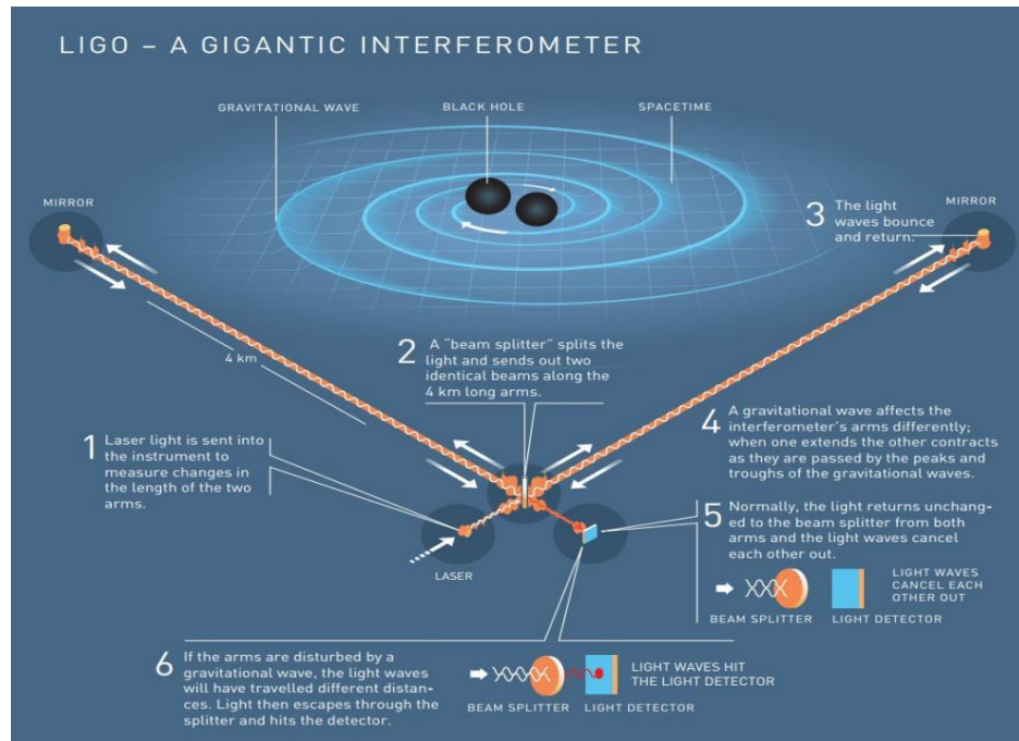
Figure 2: LIGO Interferometer: An illustration of the Laser Interferometer Gravitational-Wave Observatory (LIGO), showcasing the interferometer's design and the concept of laser interferometry used to detect gravitational waves. The world's first observed gravitational waves were created in a violent collision between two black holes, 1.3 billion lightyears away. When these waves passed the Earth, 1.3 billion years later, they had weakened considerably: the disturbance in spacetime that LIGO measured was thousands of times smaller than an atomic nucleus. Credit: LIGO
