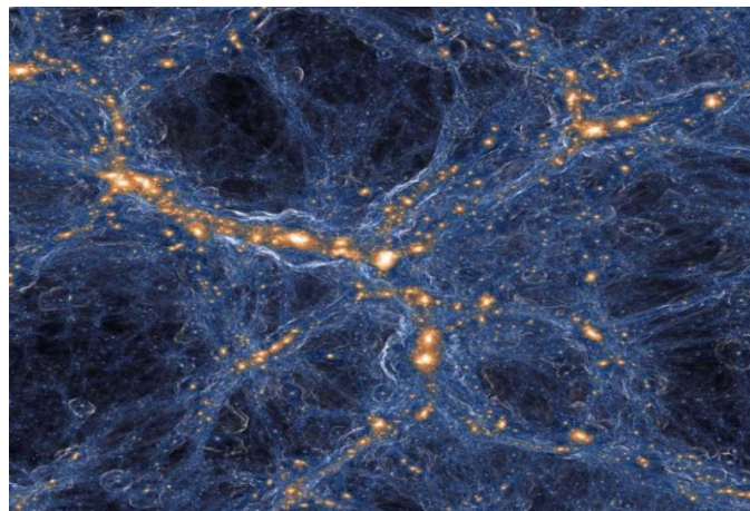
Figure 1: Dark Matter Distribution: A composite model of matter distribution (with dark matter overlay) in a galaxy formation simulation made by the TNG Collaboration. The figure demonstrates the invisible nature of dark matter and highlights its role in shaping the large-scale structure of the universe.
