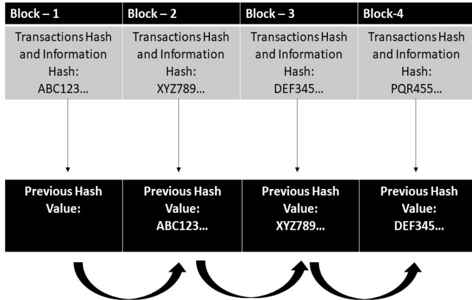
Figure1: Blockchain Architecture
