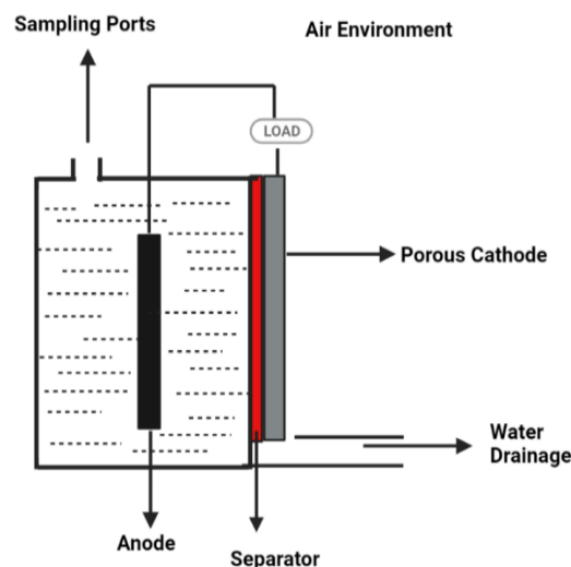
Figure 3: Single Chamber MFC: In this model both anode and Cathode Electrode are fixed into the same Chamber and connected by External Wire
