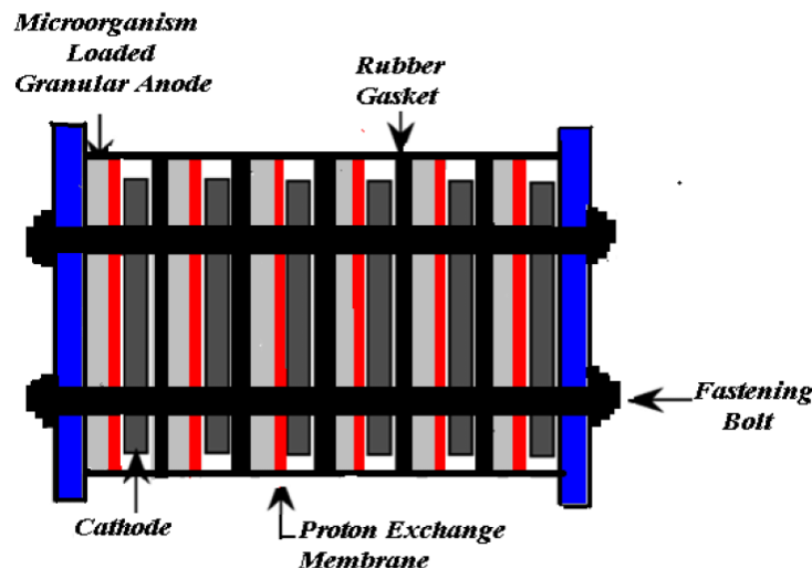
Figure 6: Schematic design of Stacked type Microbial Fuel Cell
