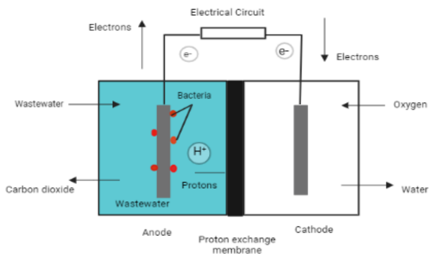
Figure 5: Two chambered MFC separated by Proton Exchange Membrane
