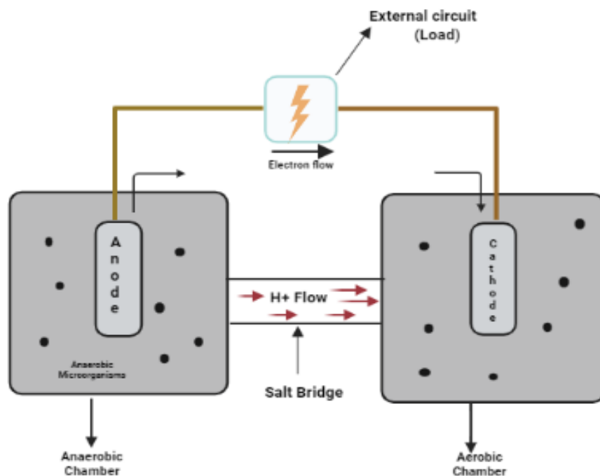
Figure 4: Two chambered MFC separated by salt bridge
