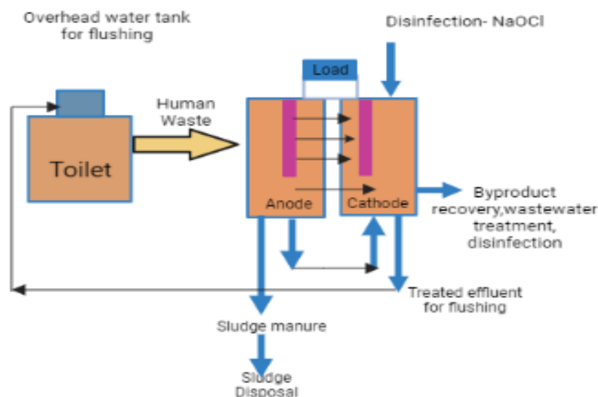
Figure 9: Schematic diagram showing the integration of Human waste in MFC technology
