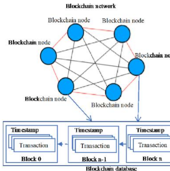
Figure 1:Blockchain architecture
