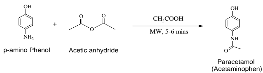
Scheme-1: Synthesis of Paracetamol and Aspirin under Microwave irradiation
