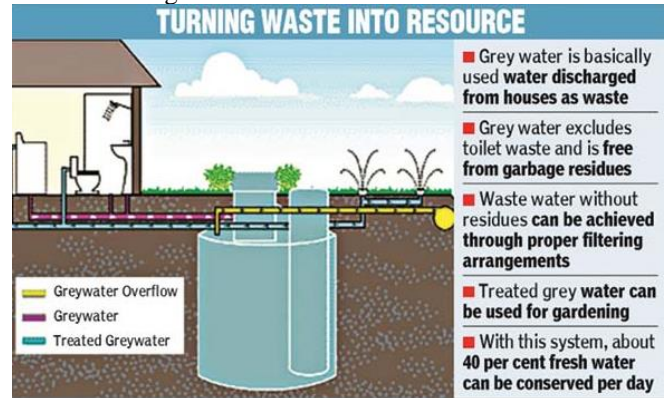
Fig 2: grey water purification [32]
