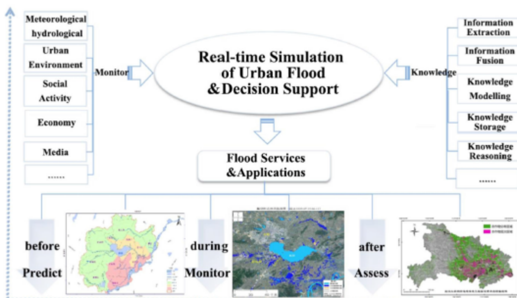
Figure 9: Flood monitoring and service platform architecture for a smart city
