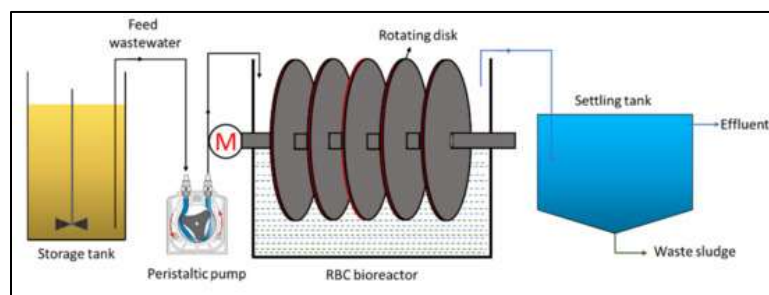
Figure 4: Schematic diagram of rotating biological contractor
