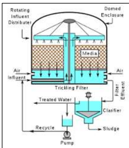
Figure 3: Schematic diagram of trickling filters
