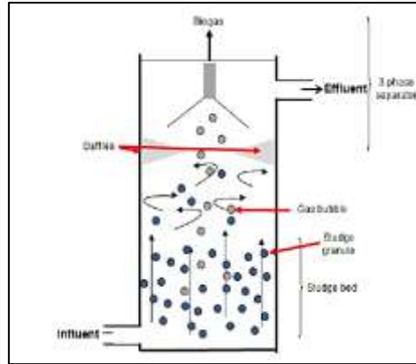
Figure 1: Schematic diagram of UASB
