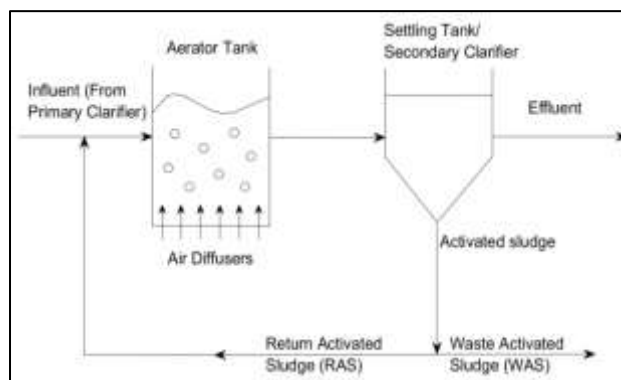
Figure 2: Schematic diagram of activated sludge process
