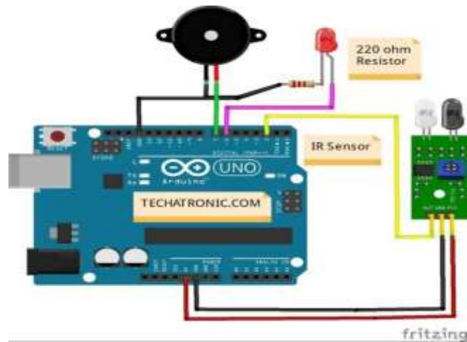
Figure 1: Circuit diagram of proposed method.
