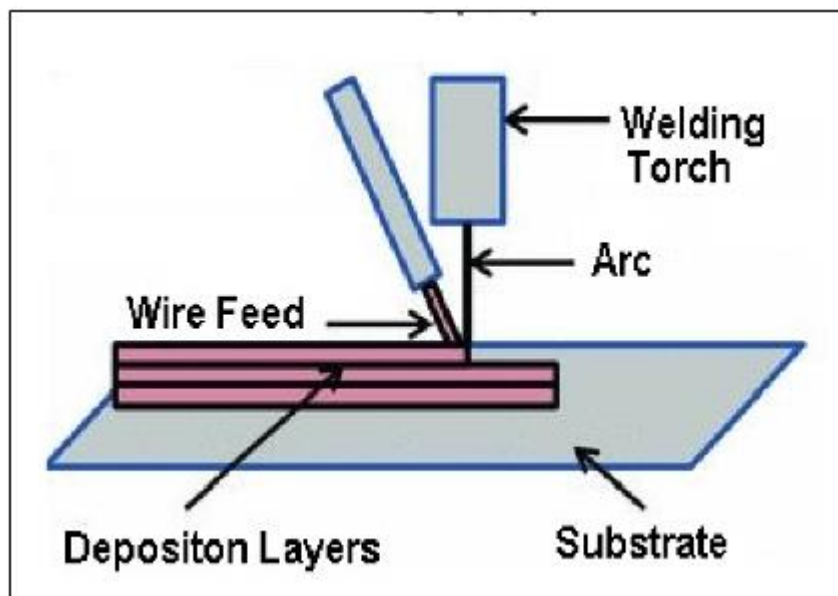
Figure 1: wire and arc additive manufacturing
